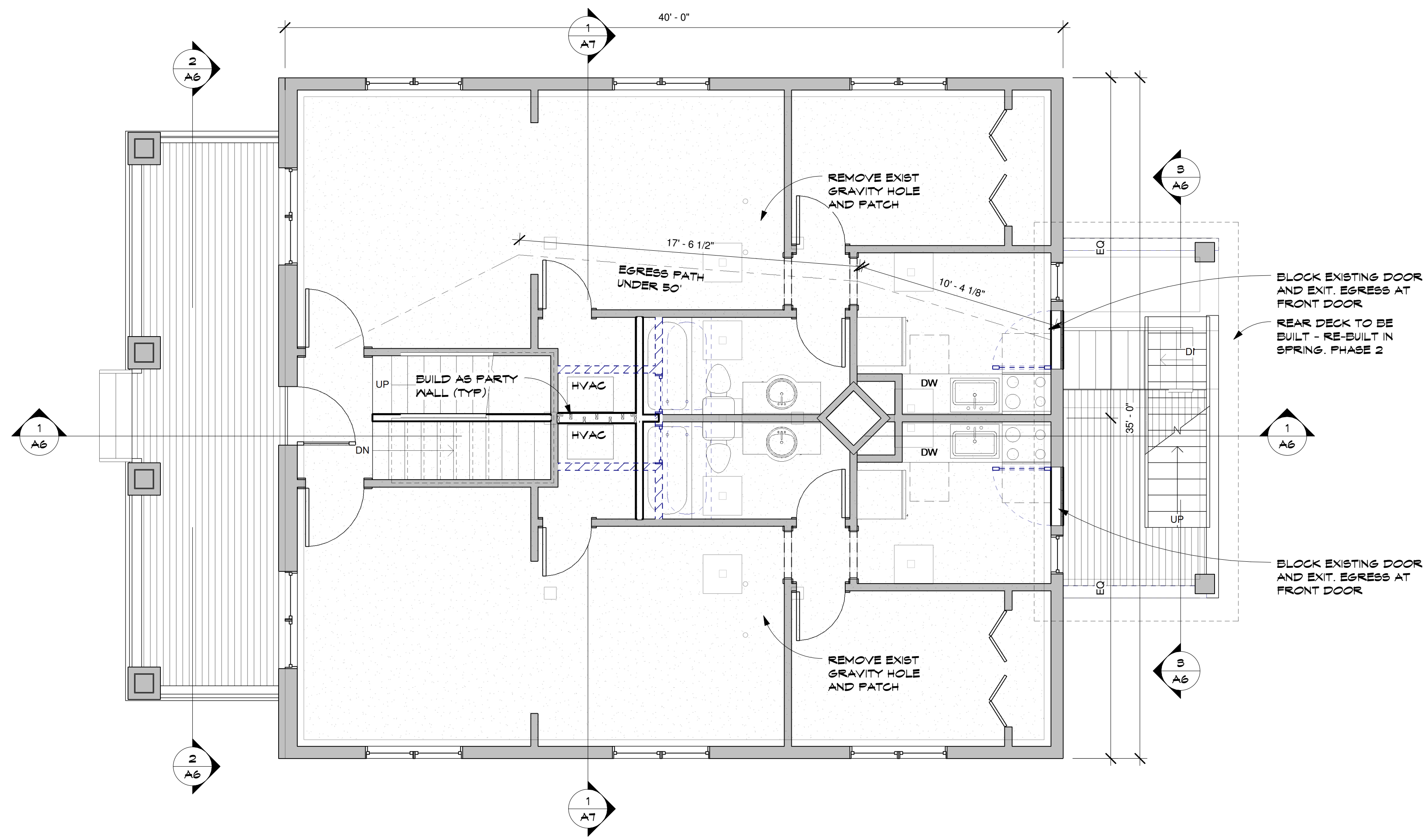
1 MAIN FLOOR A2 1/4" = 1'-0"
