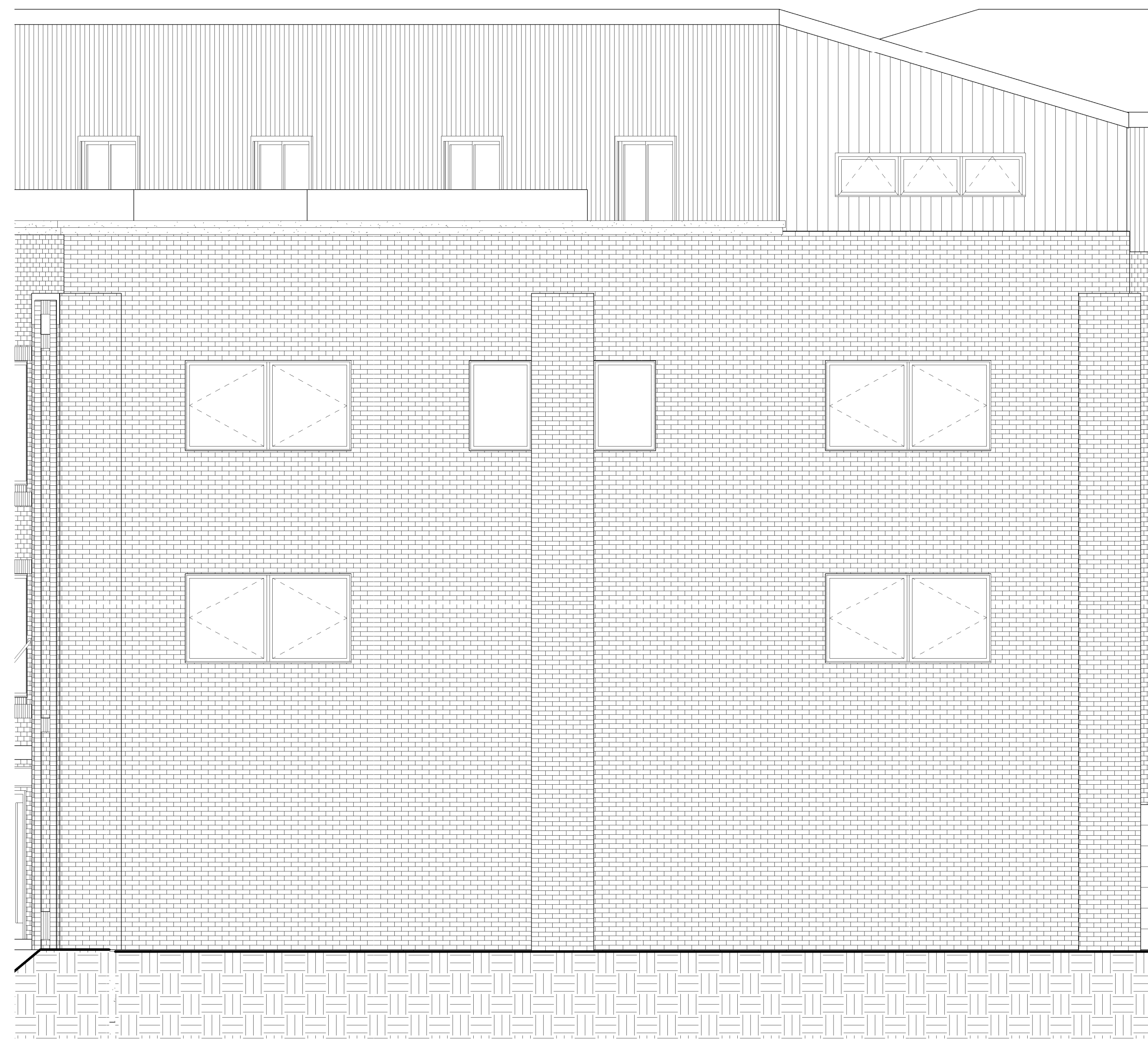
2 NORTH EXTERIOR ELEVATION BUILDING 2 A10 1/4" = 1'-0"
