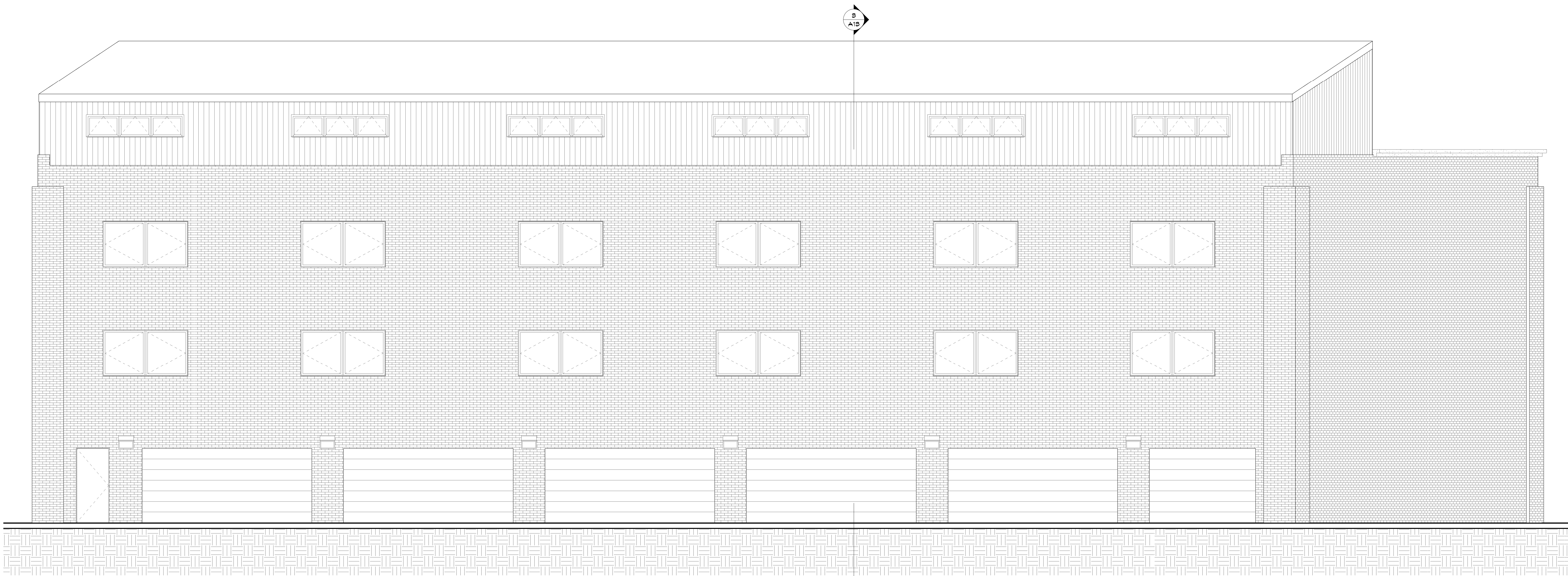
1 WEST EXTERIOR ELEVATION BUILDING 2 A10 1/4" = 1'-0"
