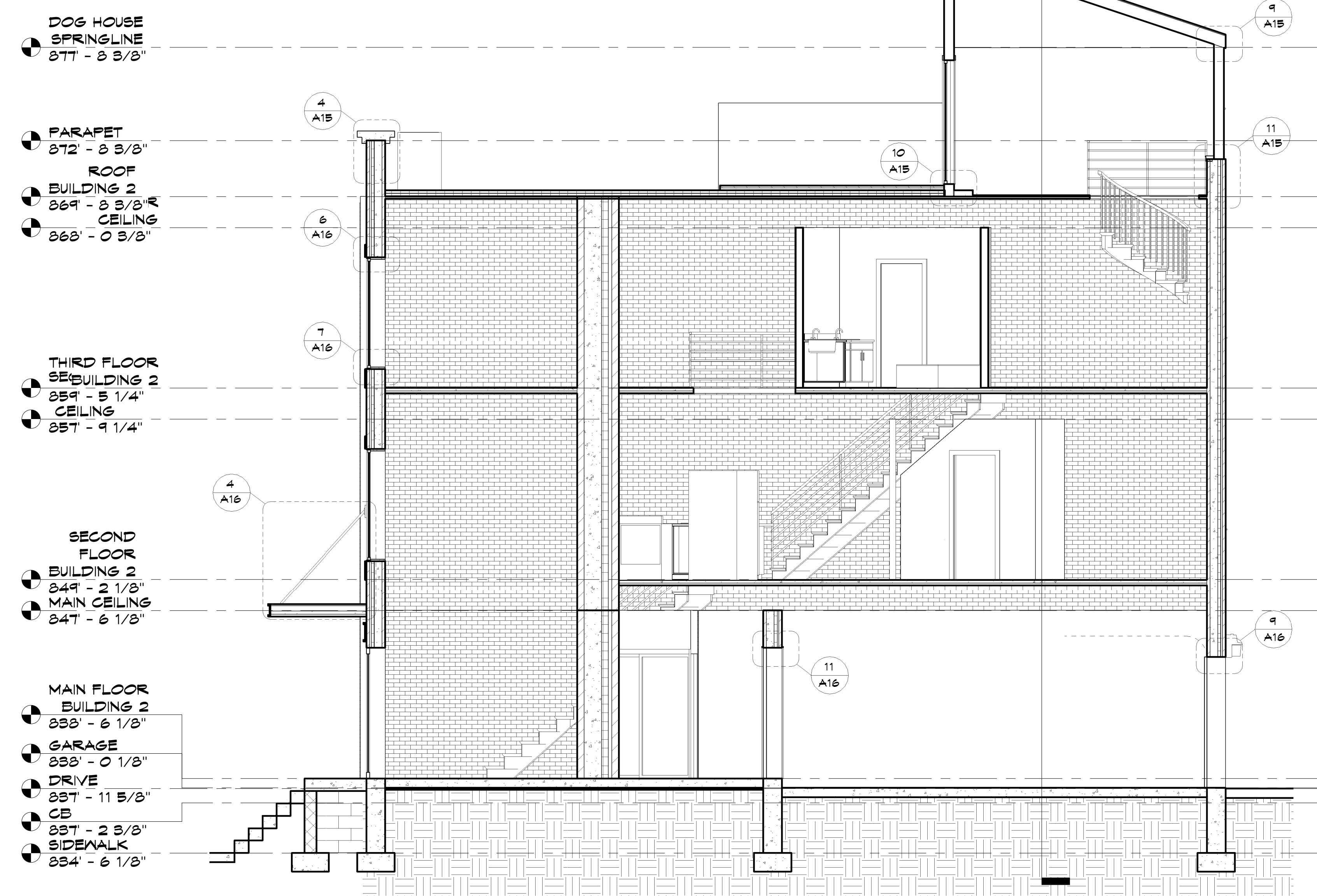
3 BUILDING SECTION-BLDG2 1/4" = 1'-0"
