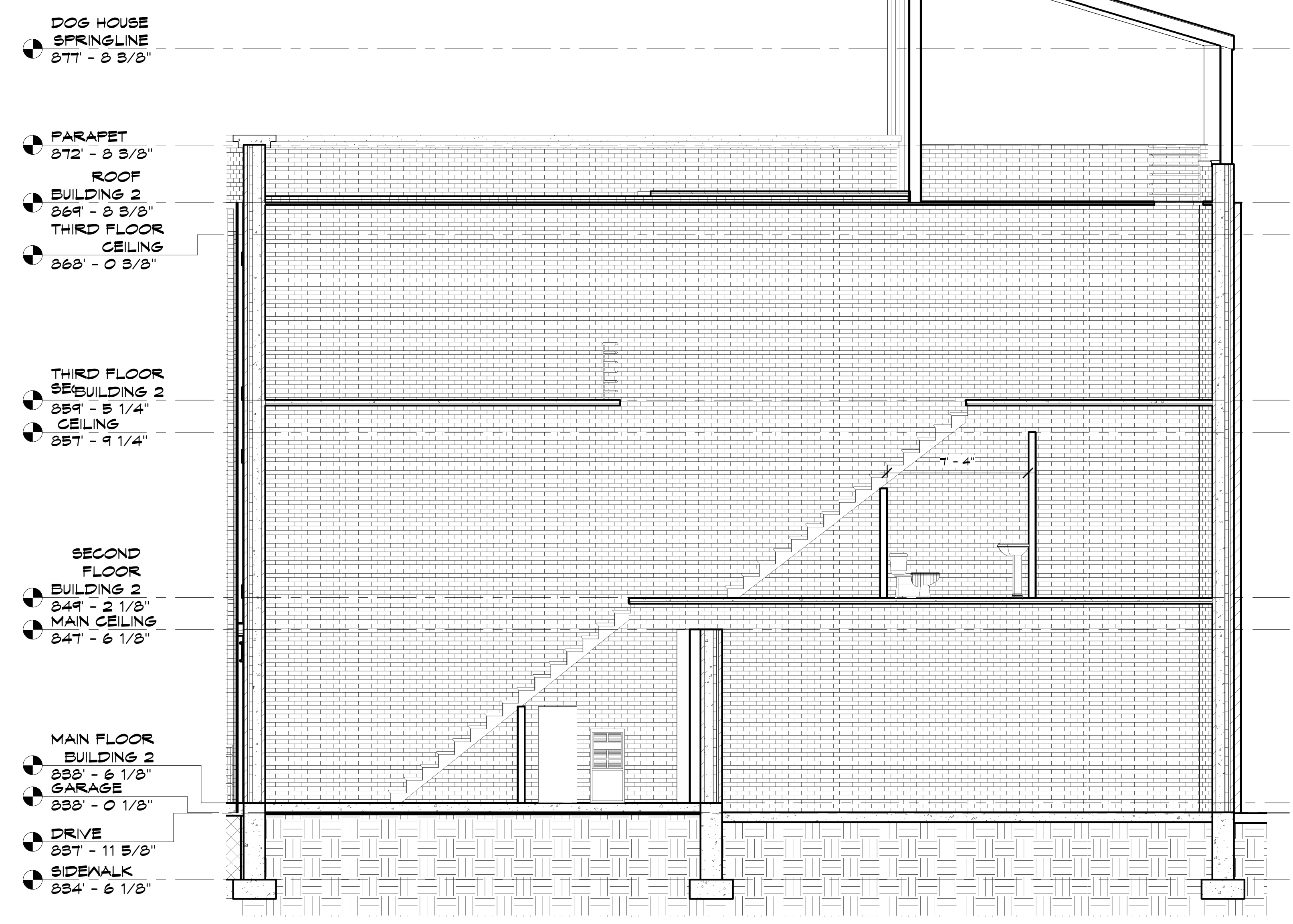
1 BUILDING SECTION AT STAIR-BLDG2 1/4" = 1'-0"
