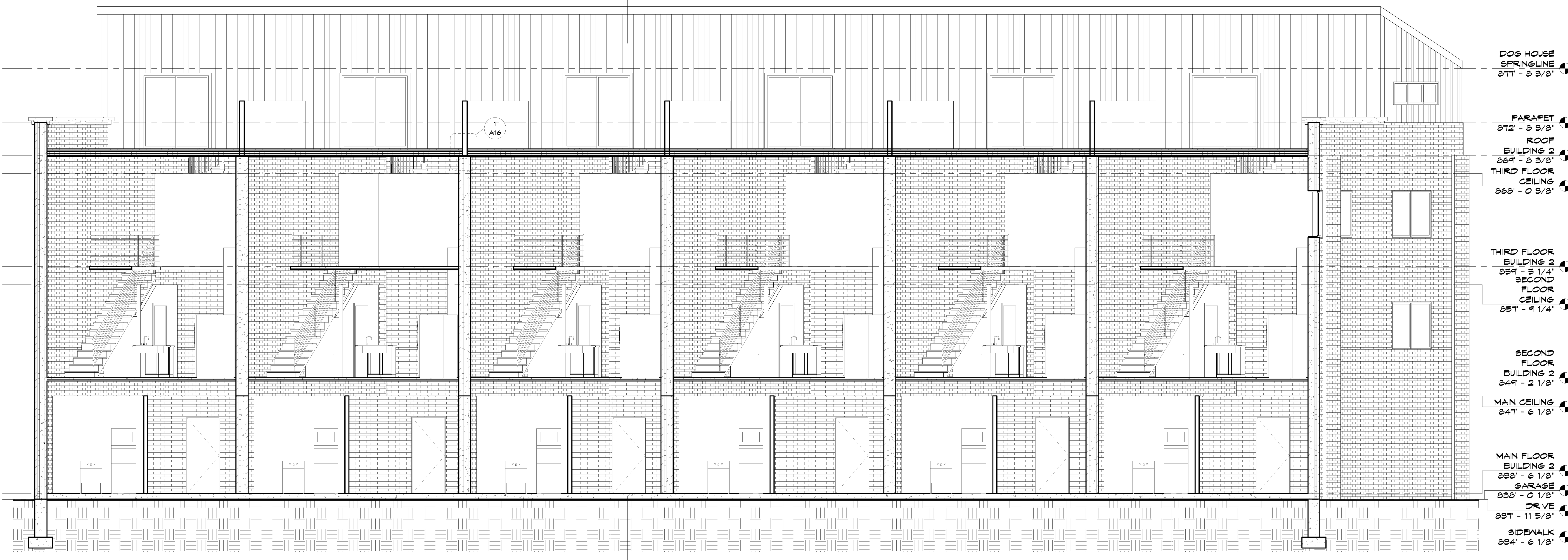
2 BUILDING SECTION AT OPENING-BLDG2 1/4" = 1'-0"
