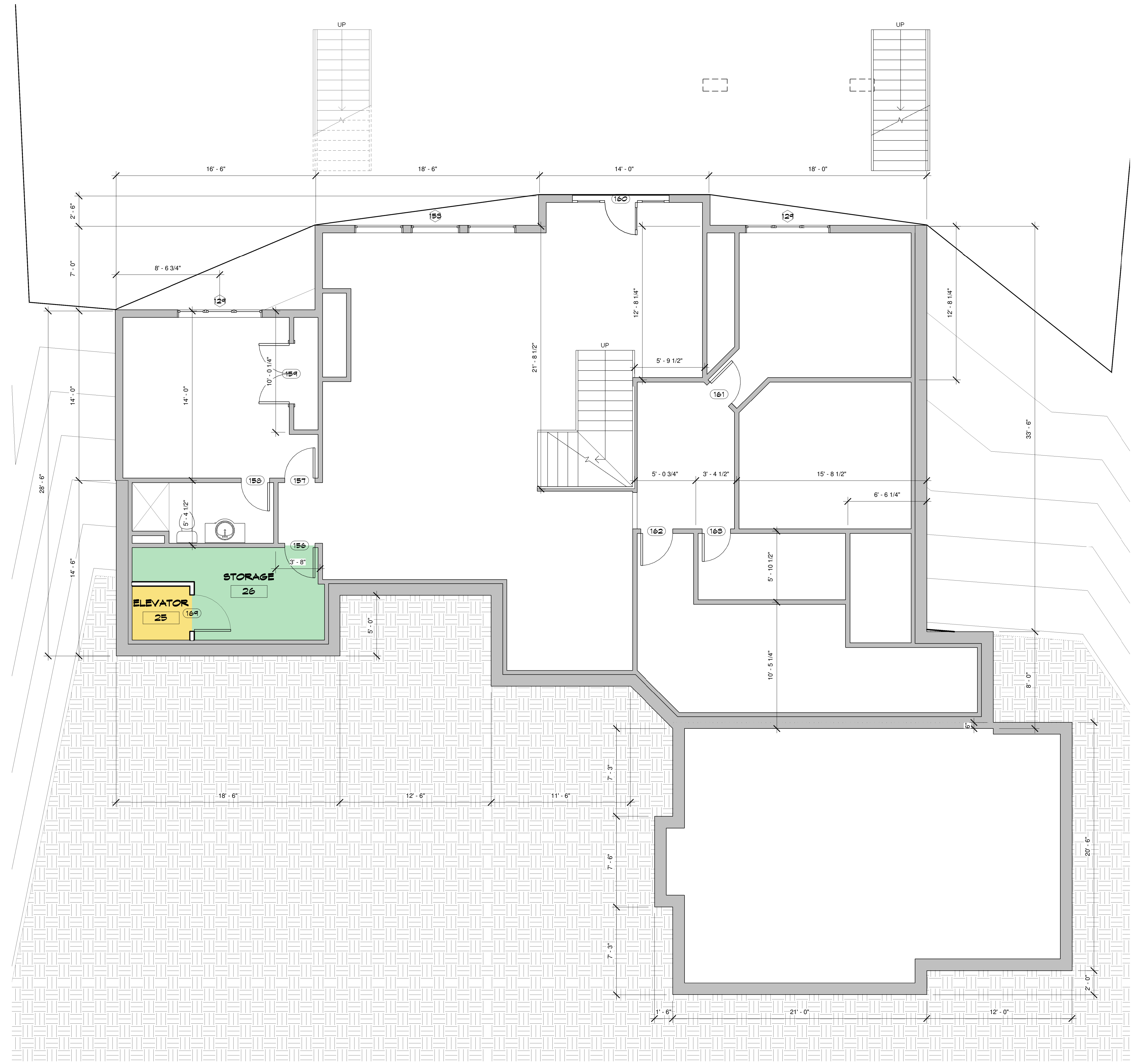
1 LOWER FLOOR A1 1/4" = 1'-0"
