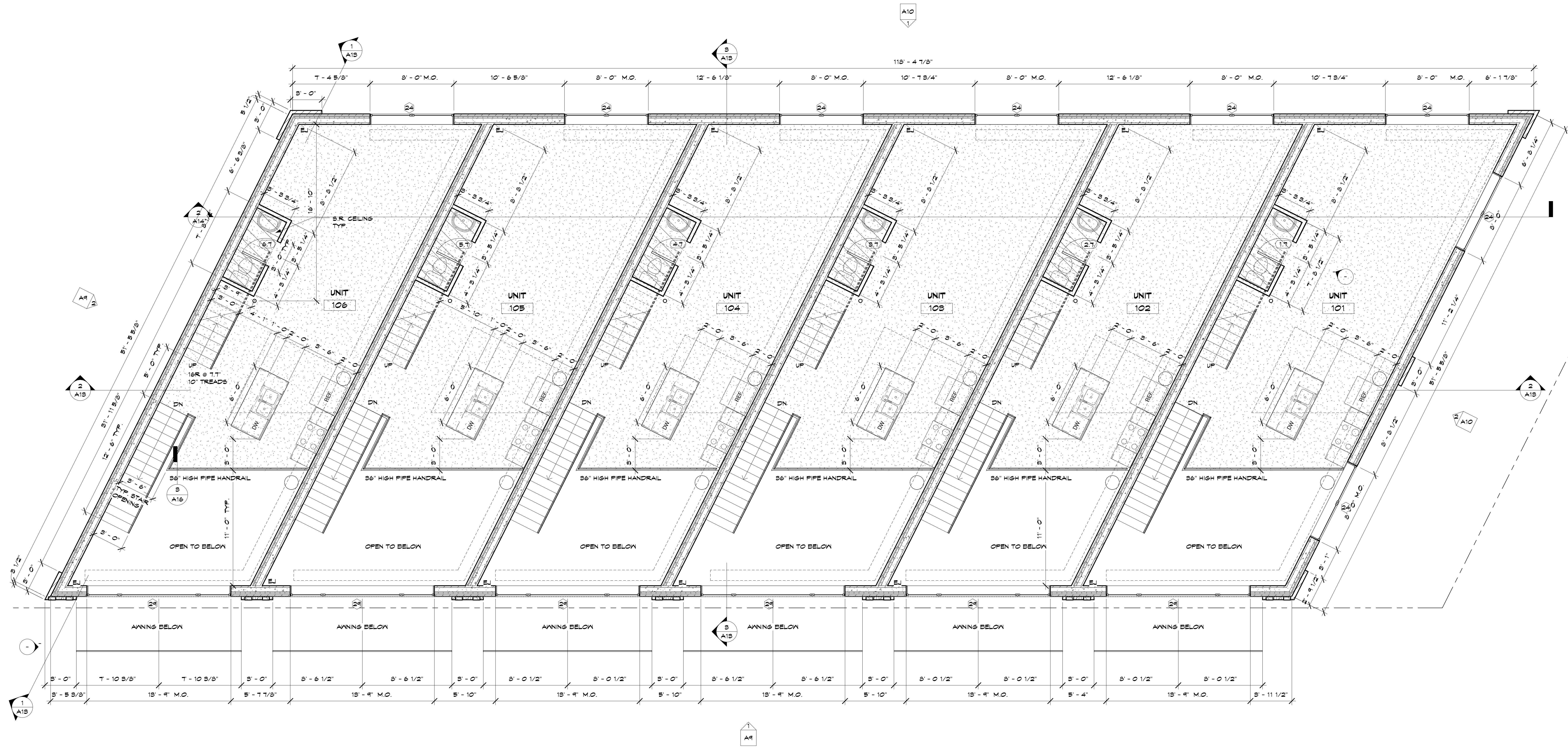
1 SECOND FLOOR BUILDING 2 A3 1/4" = 1'-0"
