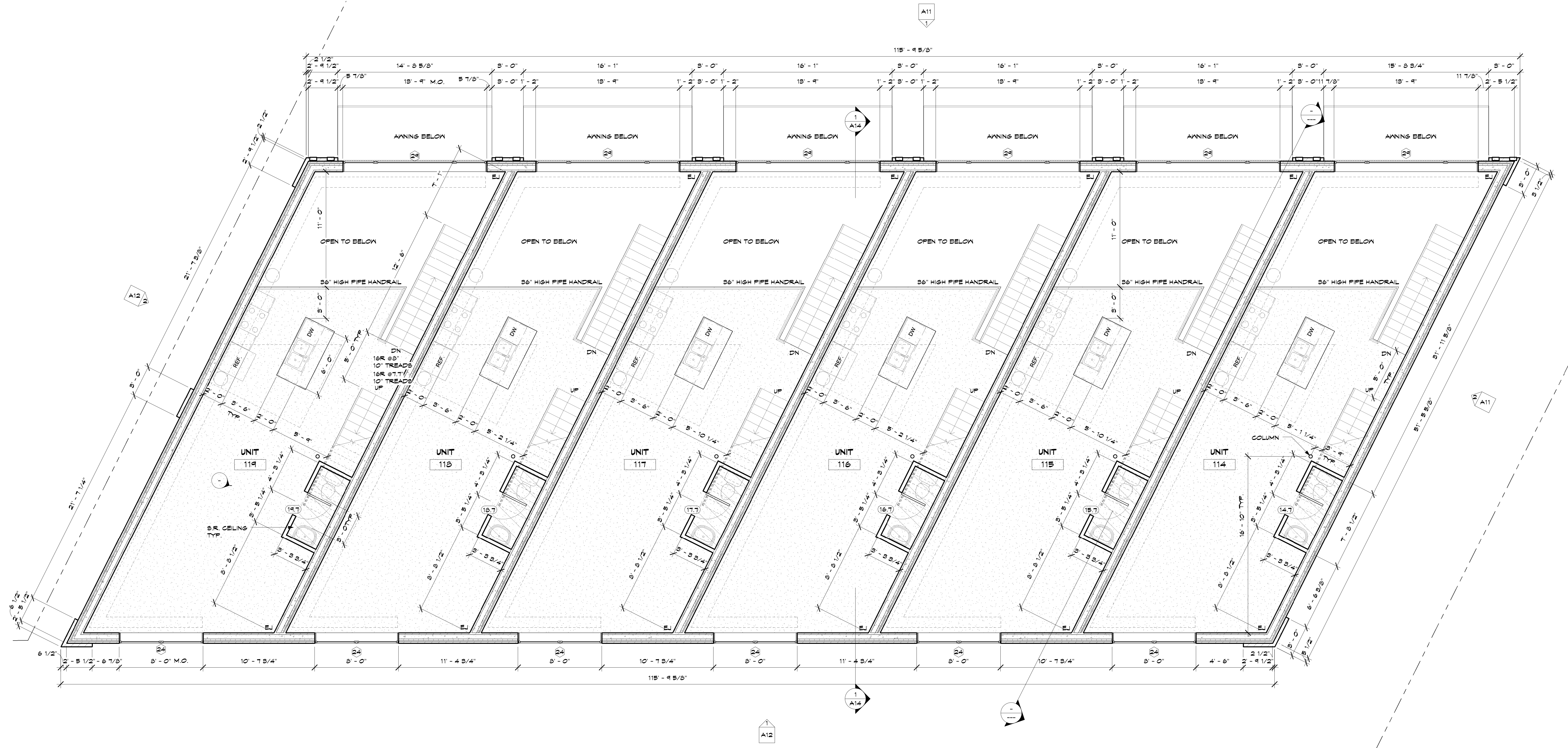
1 SECOND FLOOR BUILDING 3 A4 1/4" = 1'-0"
