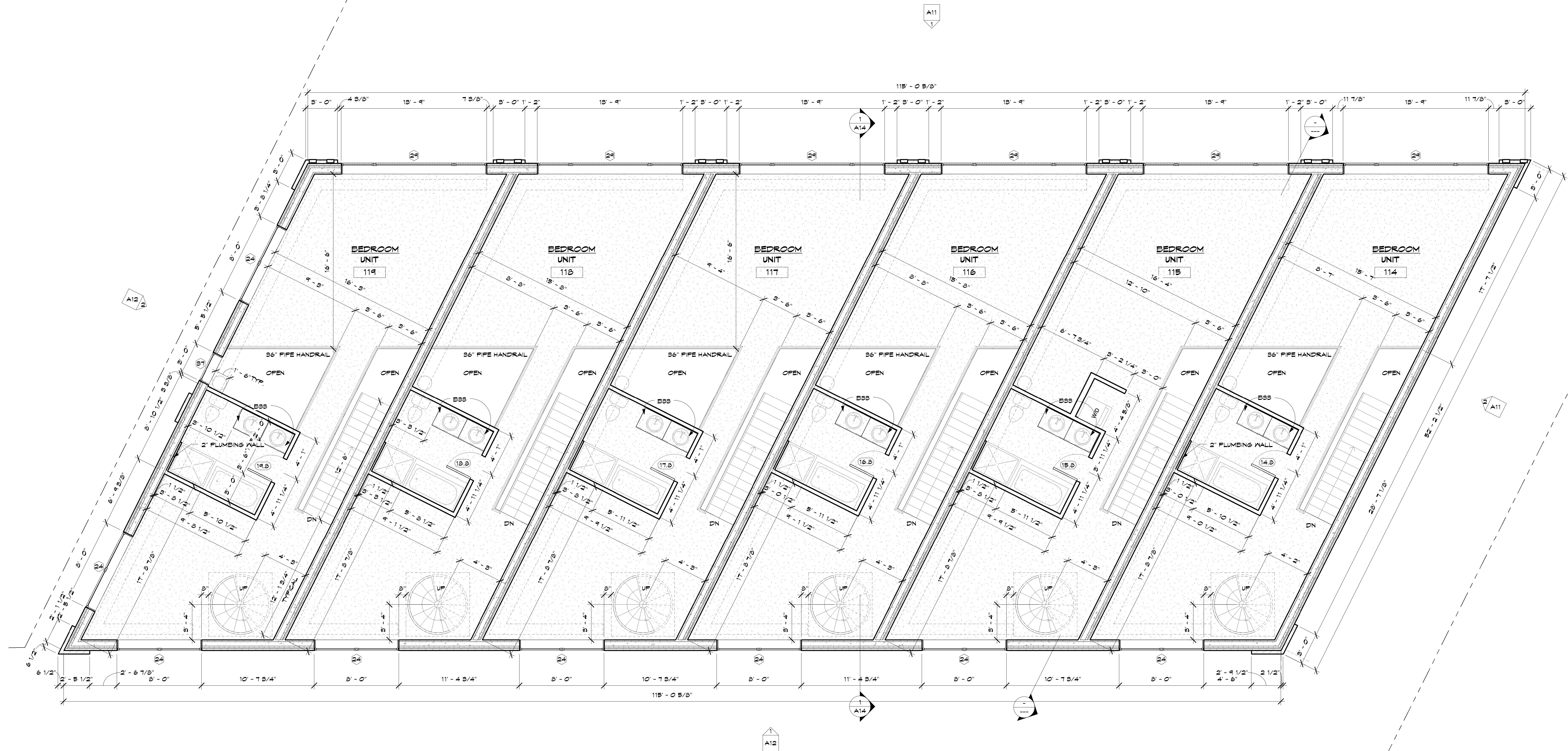
1 THIRD FLOOR BUILDING 3 A6 1/4" = 1'-0"
