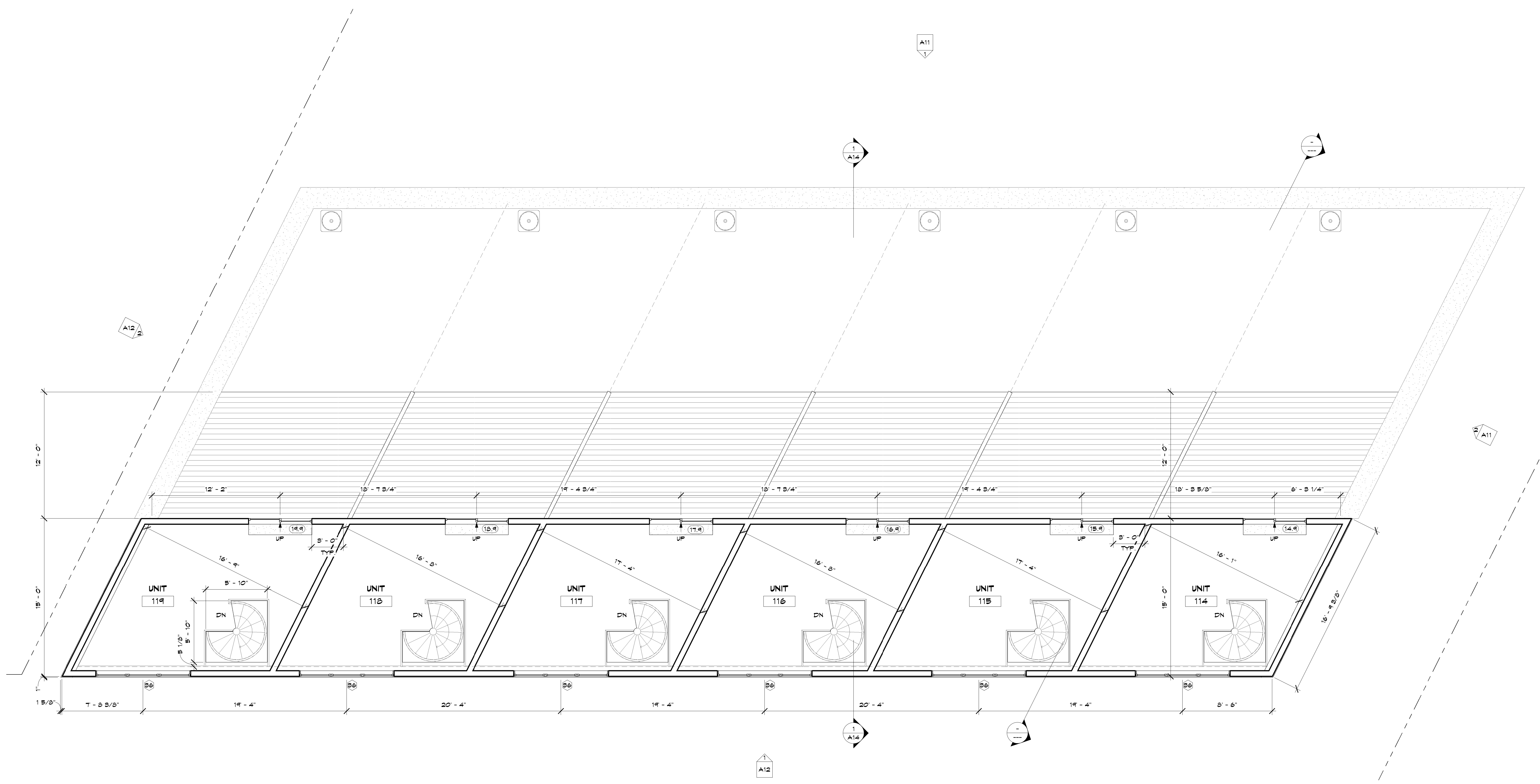
1 ROOF BUILDING 3 A8 1/4" = 1'-0"
