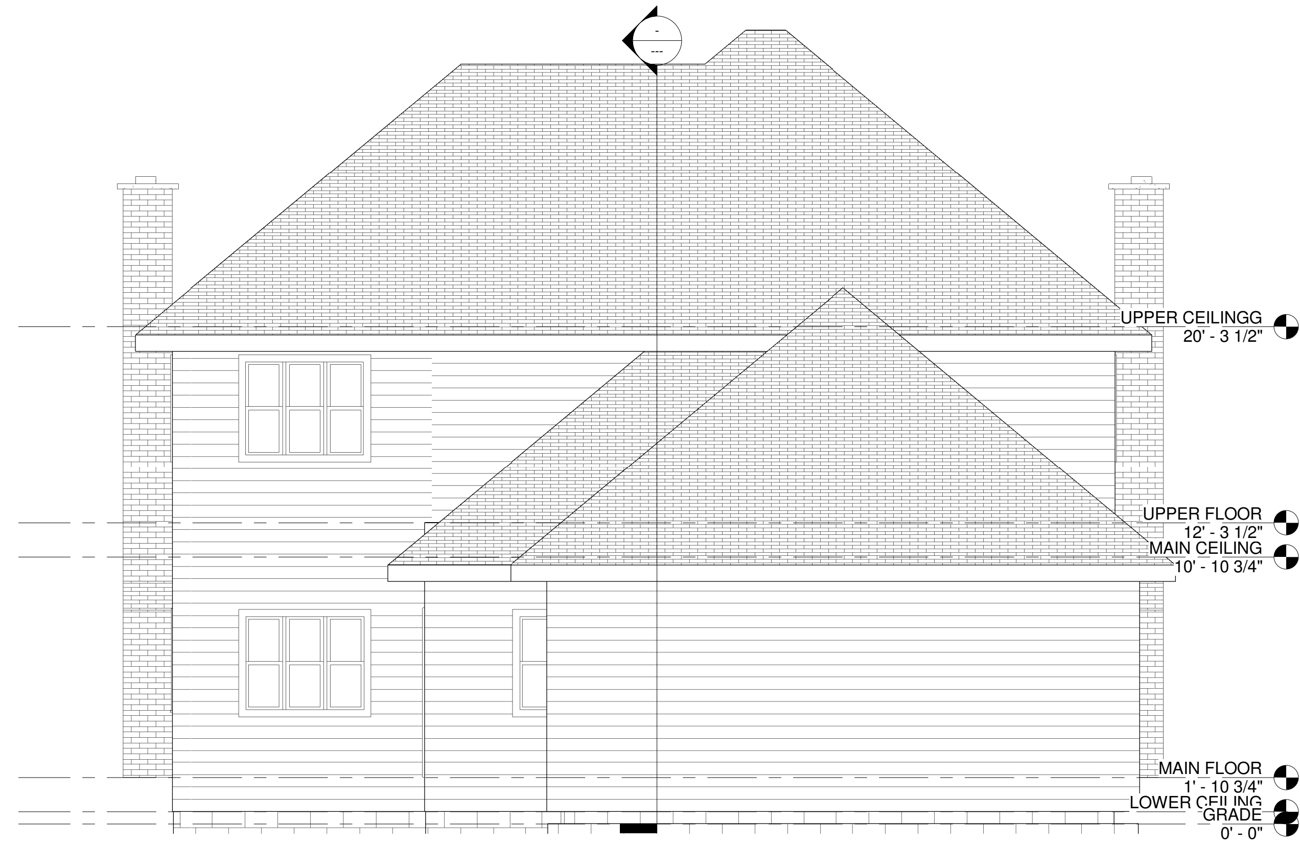
② North 1/4" = 1'-0"
