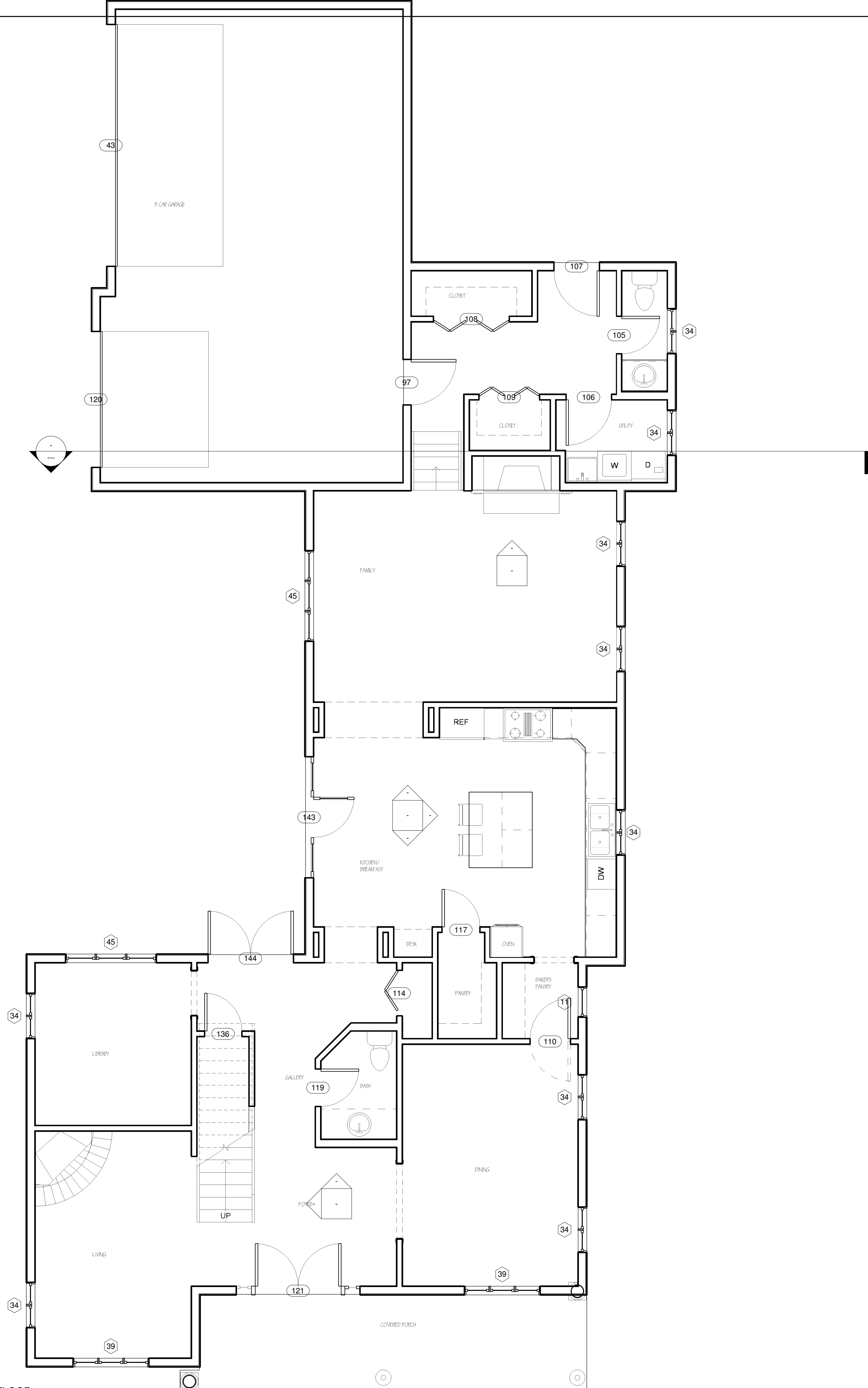
1 MAIN FLOOR 1/4" = 1'-0"
