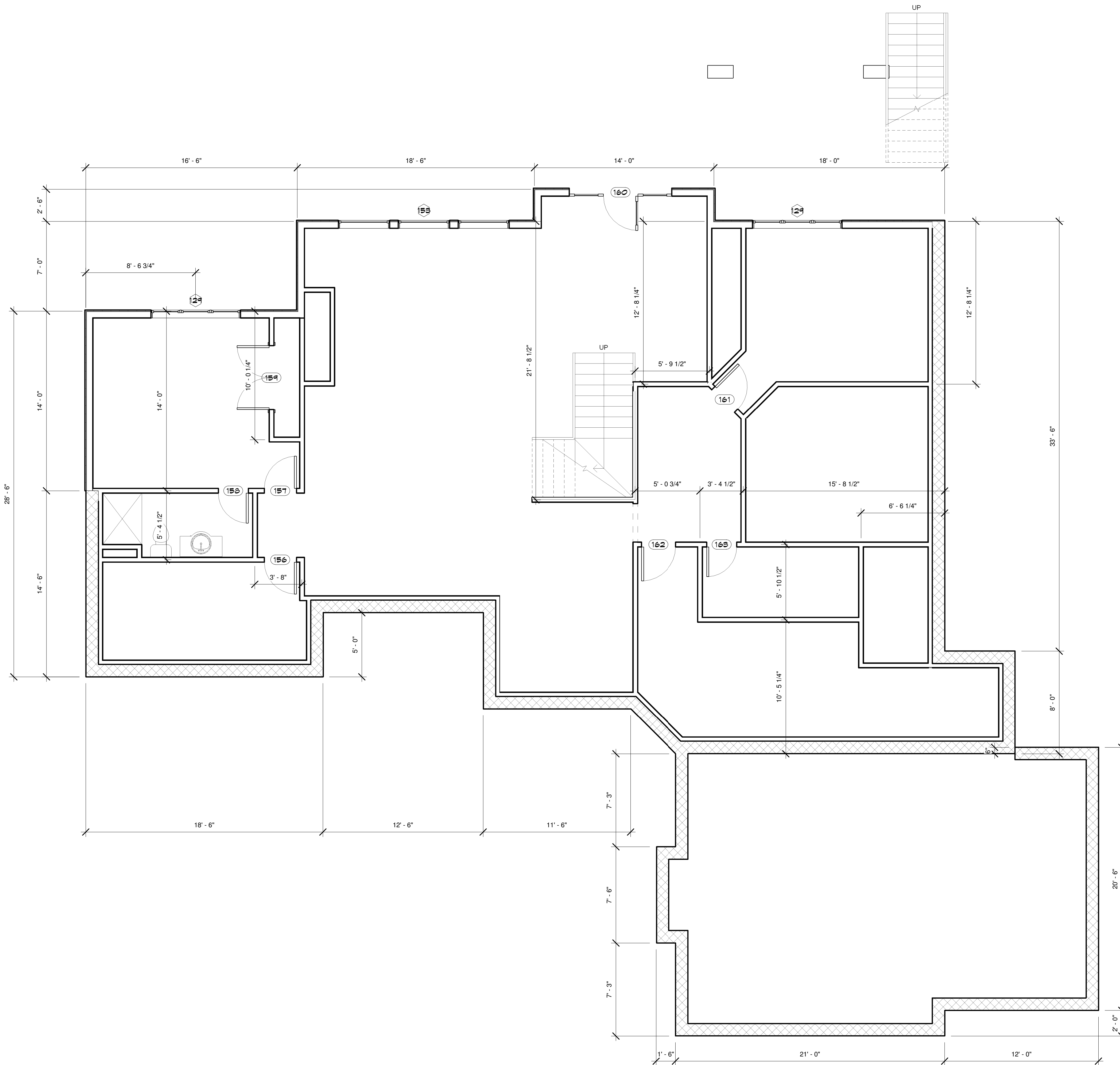
1 EXISTING LOWER FLOOR A1 1/4" = 1'-0"
