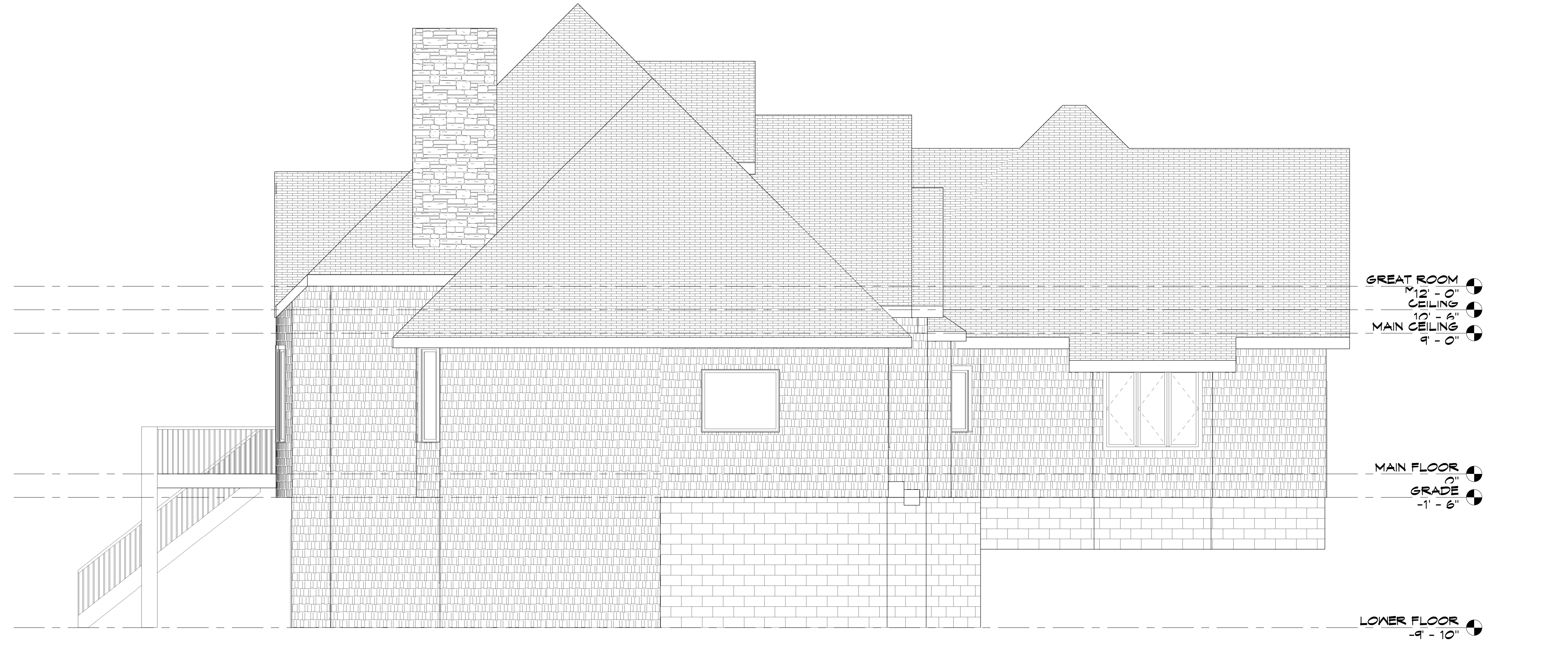
2 WEST EXIST AS 1/4" = 1'-0"
