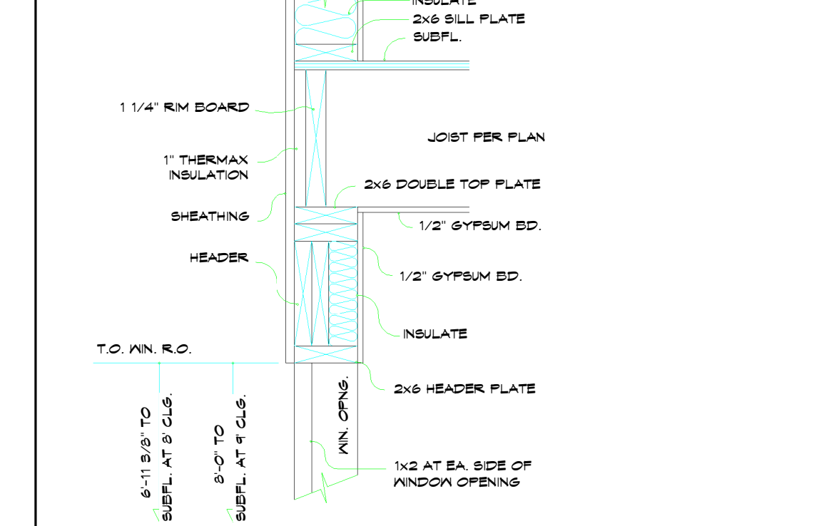
5 DETAIL AT TYPICAL HEADER 1" = 1'-0"
