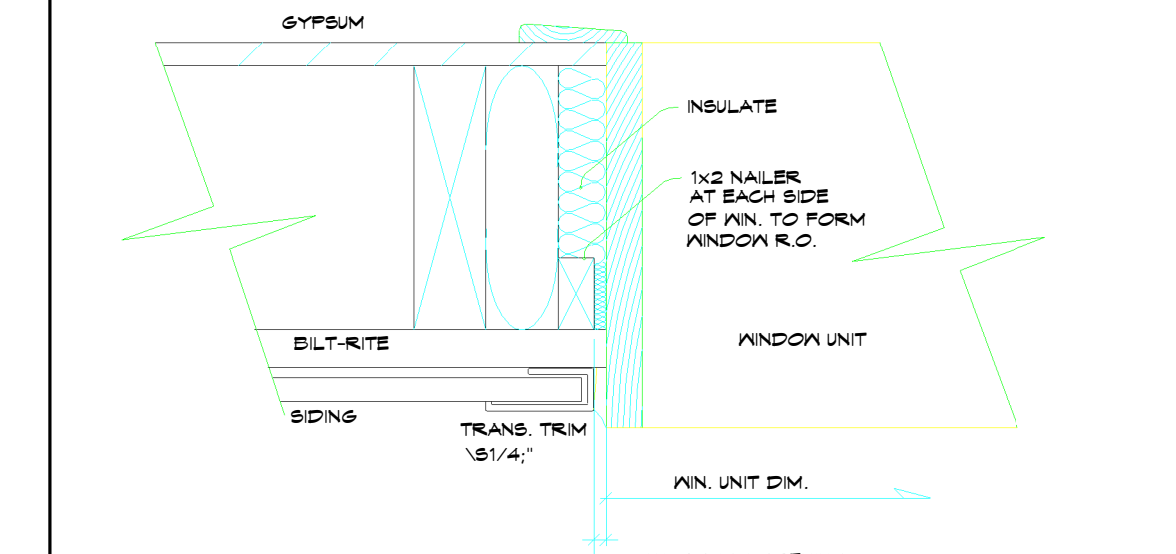
7 DETAIL AT WINDOW NAILER 1" = 1'-0"
