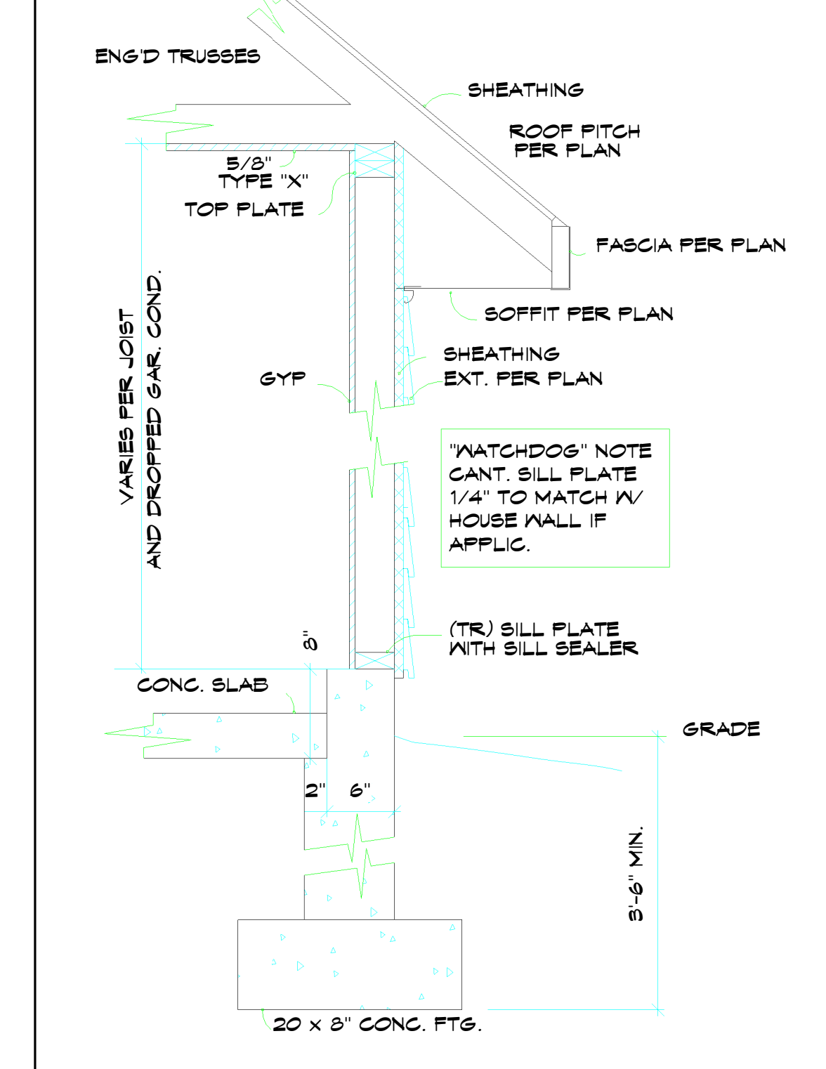
2 DETAIL AT GARAGE WALL 1" = 1'-0"
