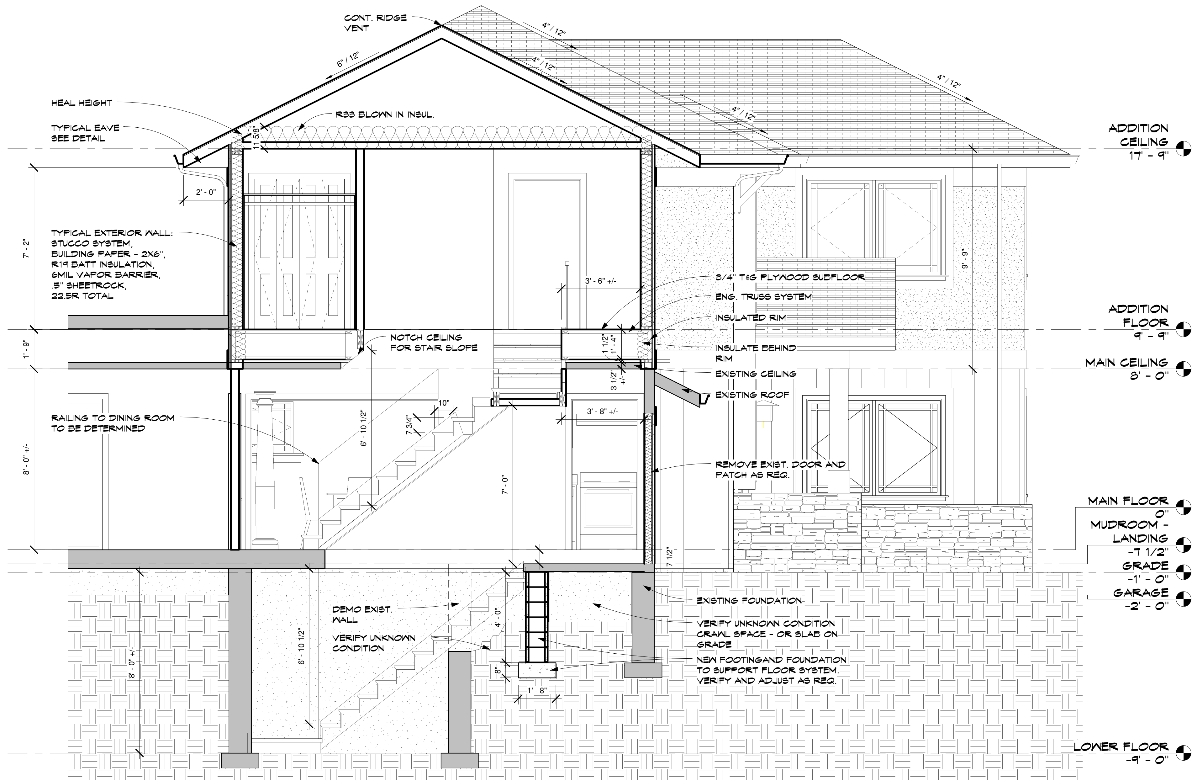
1 STAIR SECTION 1 A6 3/8" = 1'-0"
