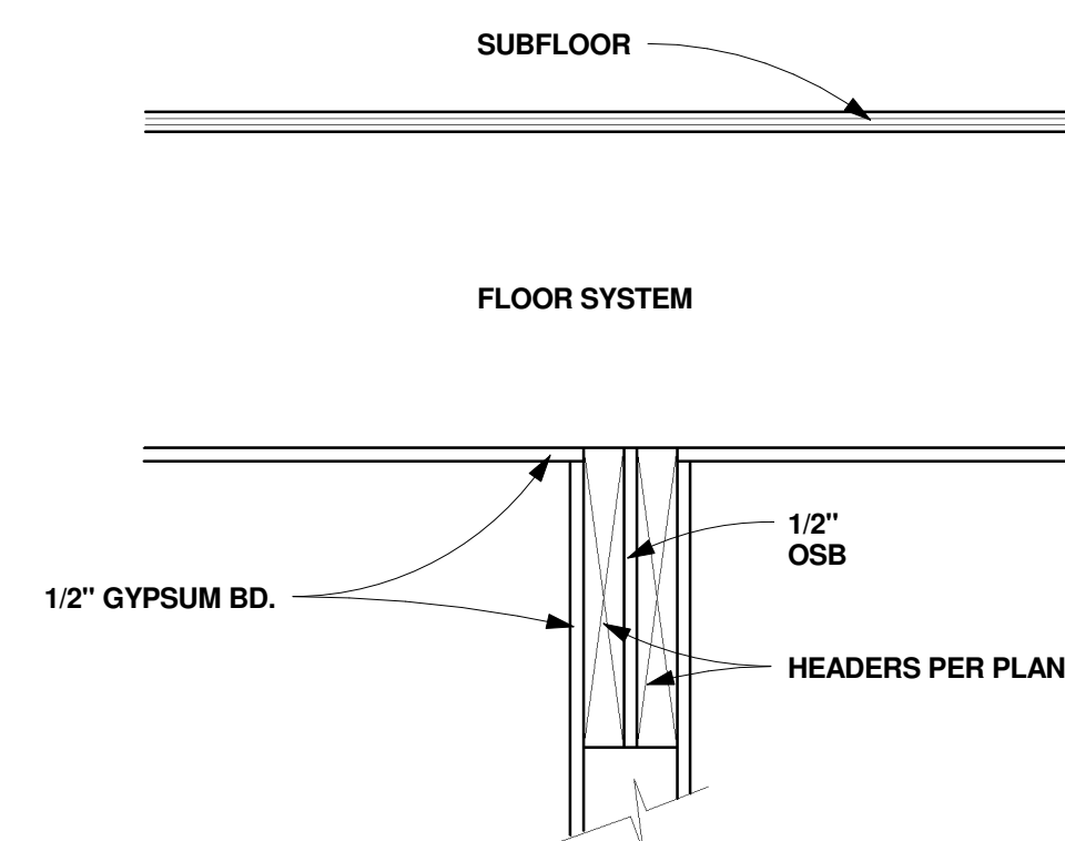
7 DETAIL AT DROPPED HEADER A8 1 1/2" = 1'-0"
