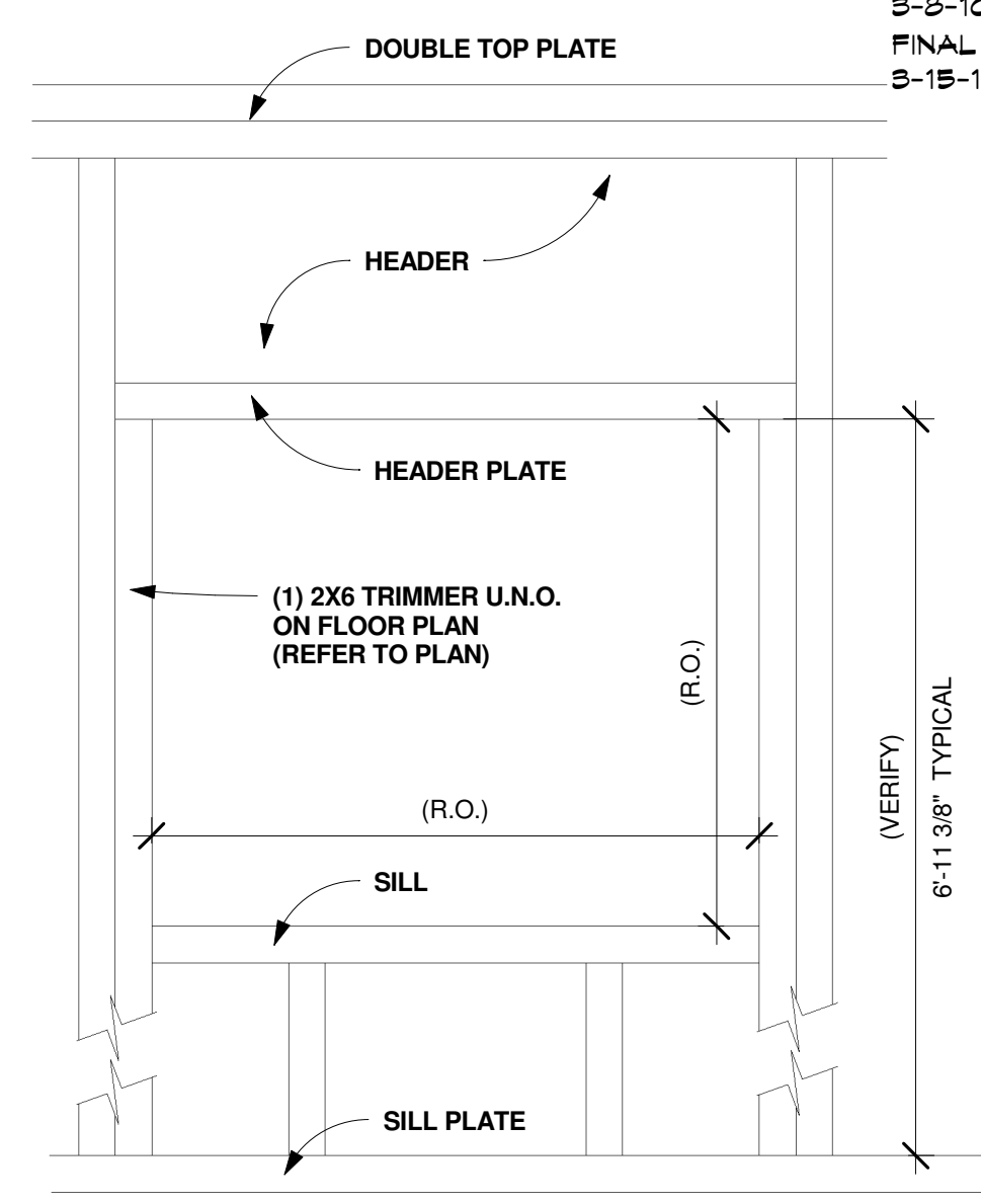
1 WINDOW FRAMING DETAIL A8 1 1/2" = 1'-0"
