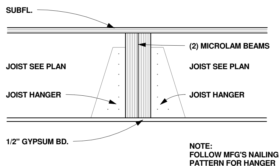
8 DETAIL AT FLUSH HEADER A8 1 1/2" = 1'-0"
