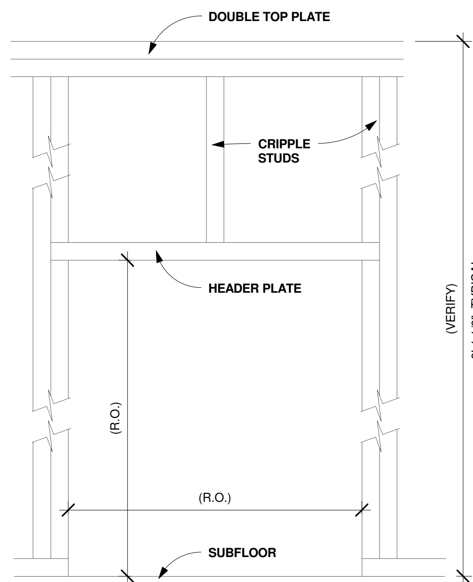
2 DOOR FRAMING DETAIL A8 1 1/2" = 1'-0"
