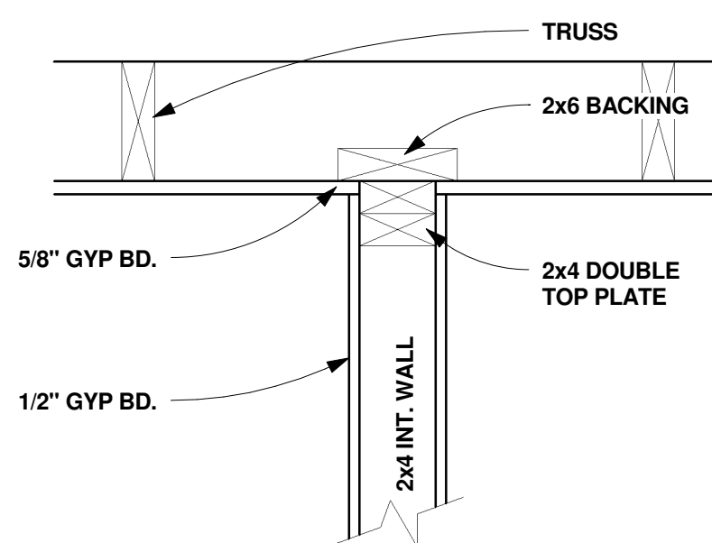
6 DETAIL AT CORNER NAILER A8 1 1/2" = 1'-0"
