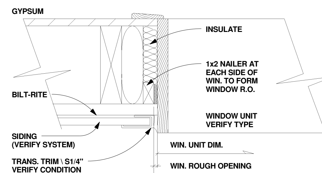
1 WINDOW FRAMING DETAIL A8 1 1/2" = 1'-0"
