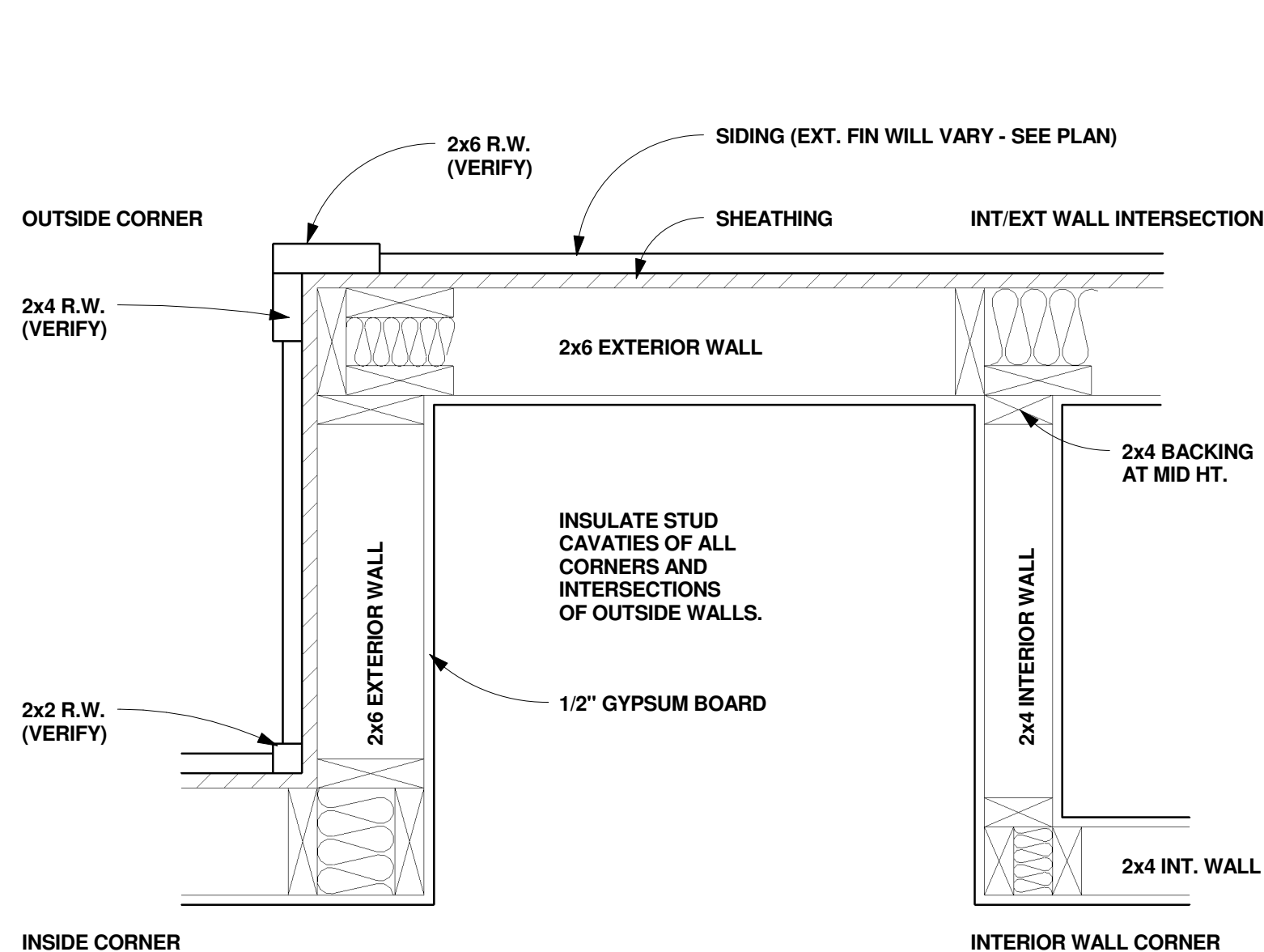
3 TYPICAL FRAMING DETAIL A8 1 1/2" = 1'-0"
