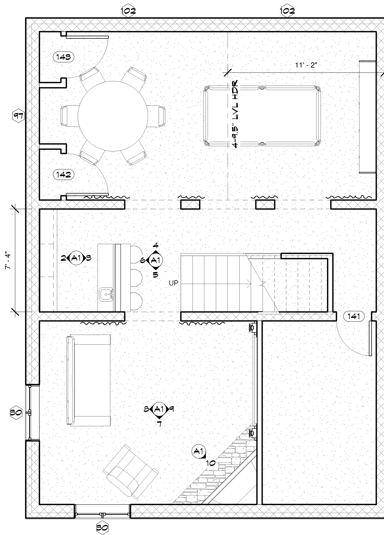
1 LOWER FLOOR A1 1/4" = 1'-0"
