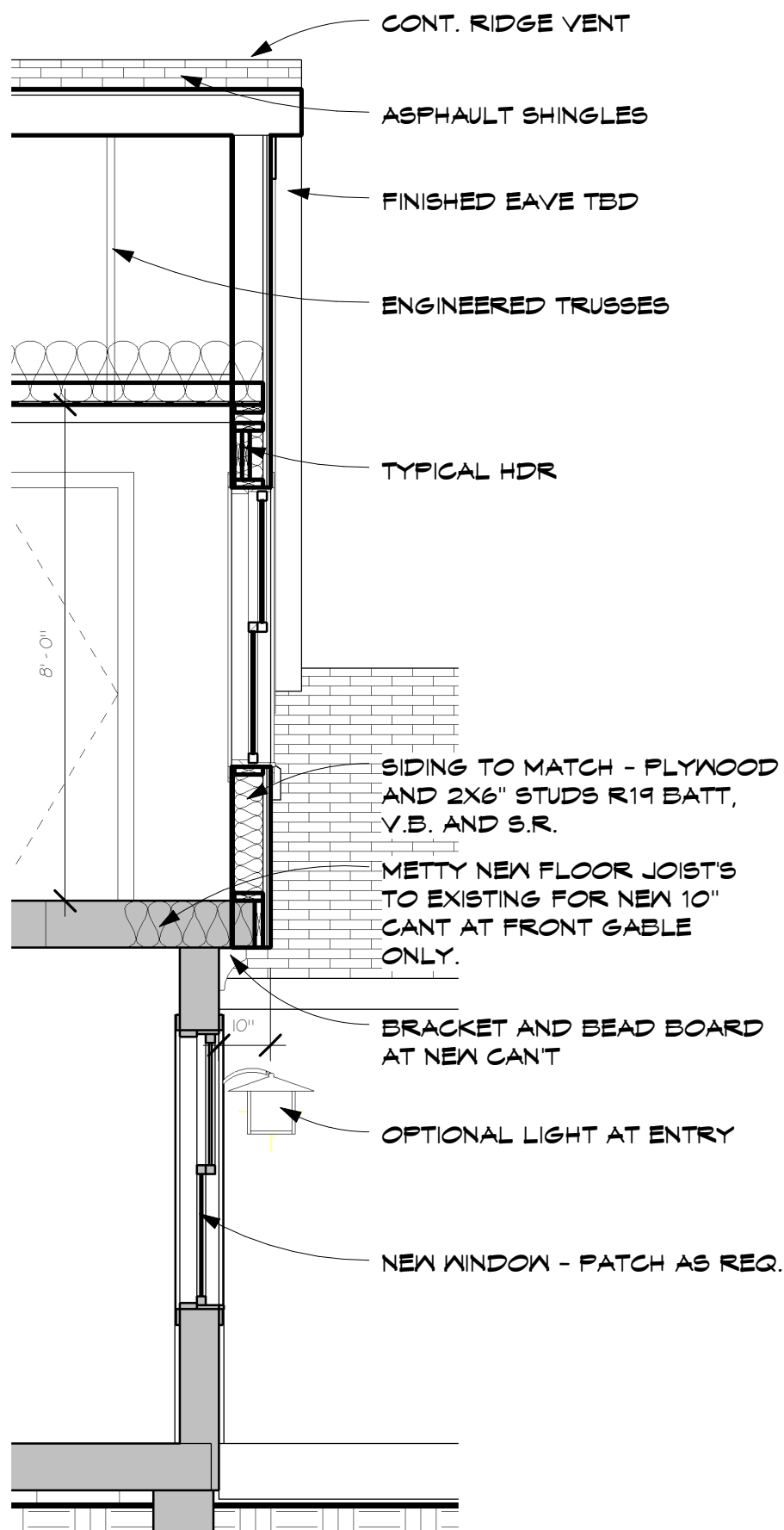
4 GABLE WALL DETAIL A2 3/8" = 1'-0"
