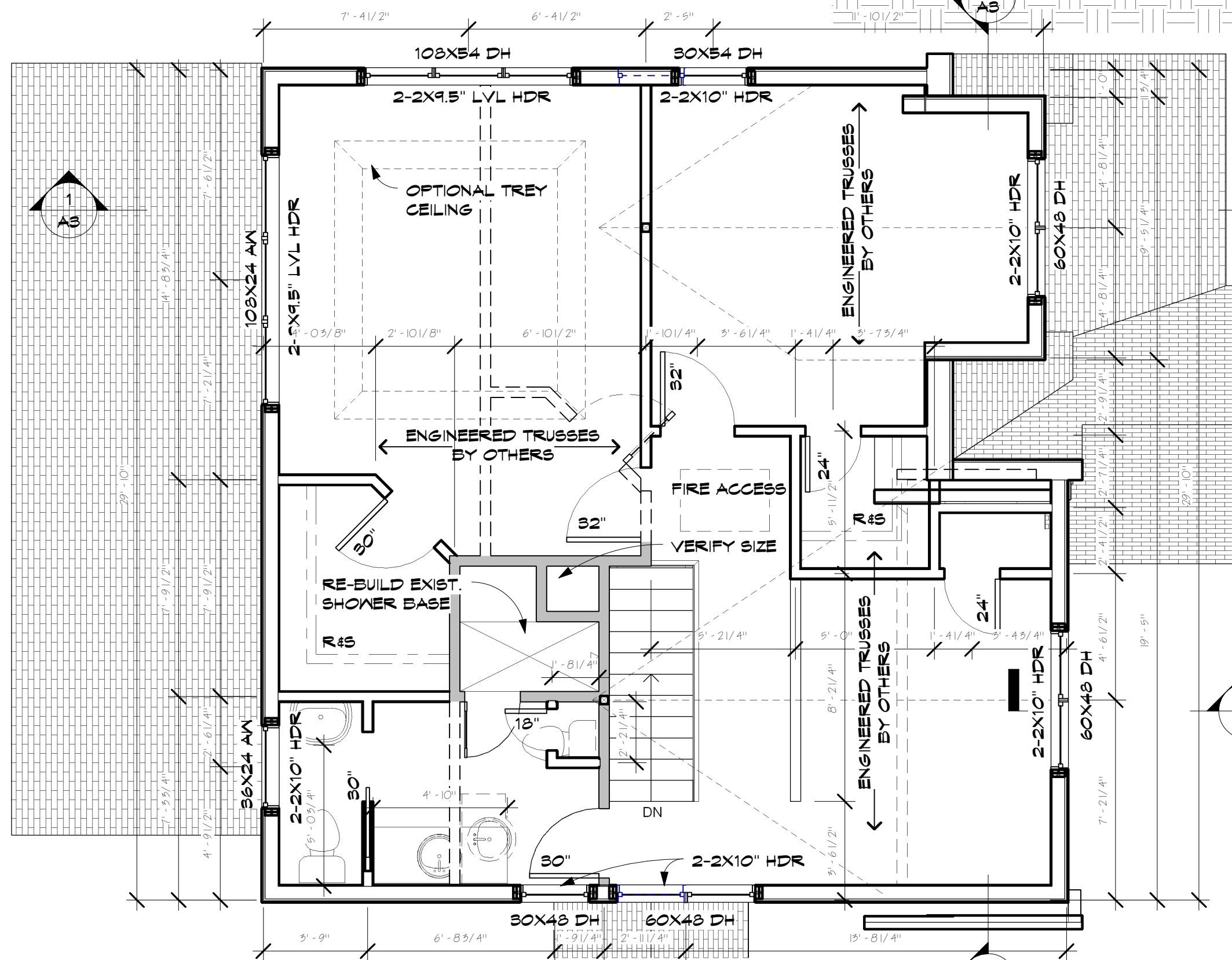
3 2ND FLOOR A1 1/4" = 1'-0"
