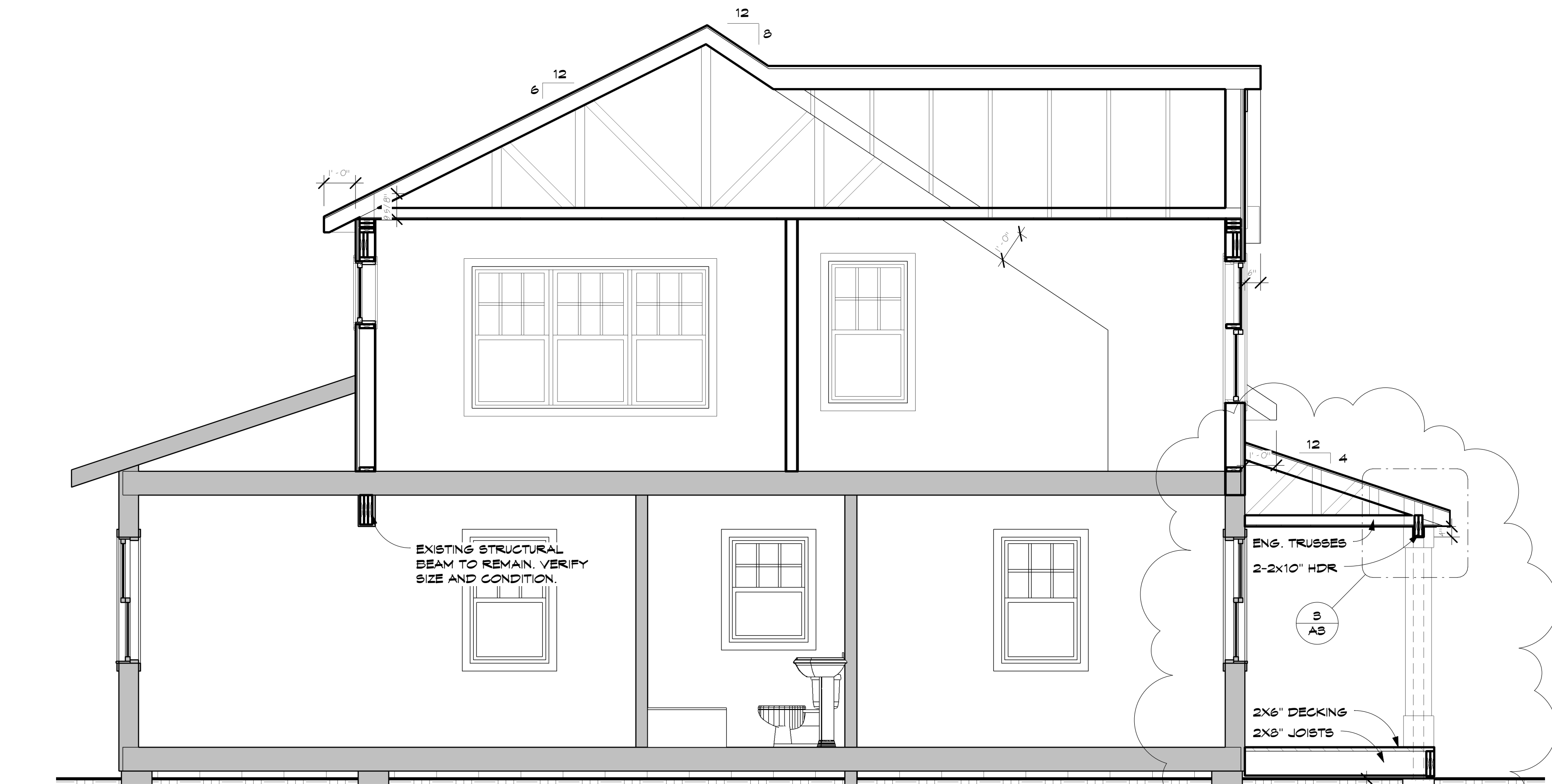
1 BUILDING SECTION 1 A3 3/8" = 1'-0"
