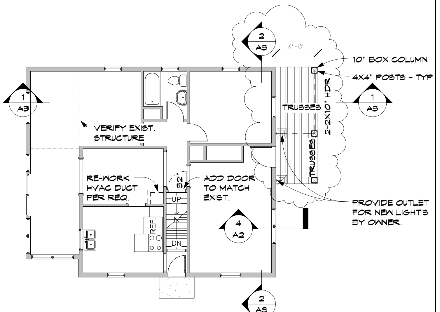
2 MAIN FLOOR A1 1/8" = 1'-0"
