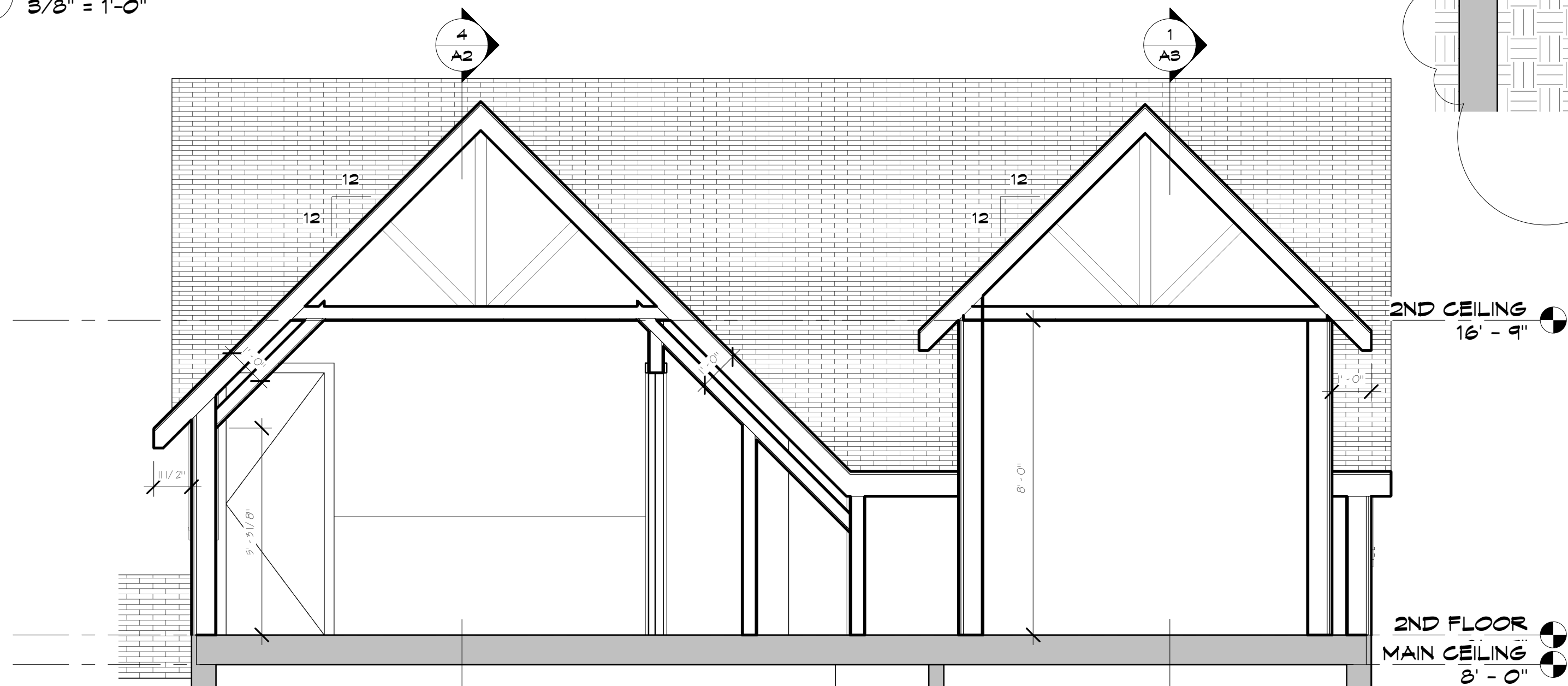
2 BUILDING SECTION 2 A3 3/8" = 1'-0"
