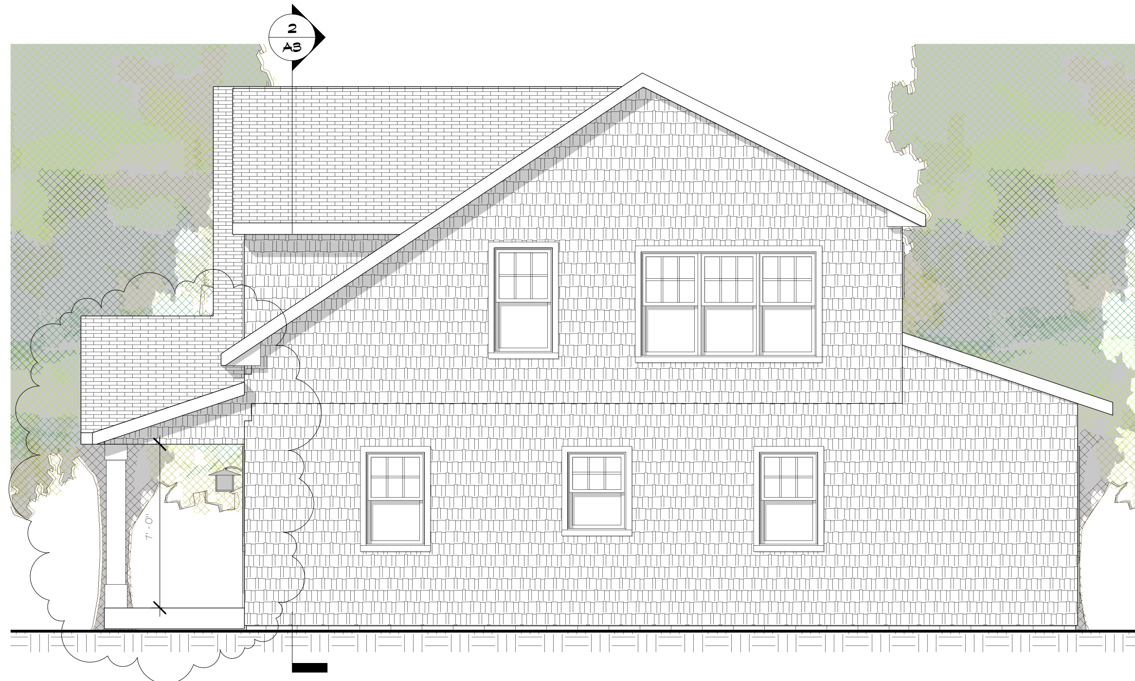
2 NORTH A2 1/4" = 1'-0"
