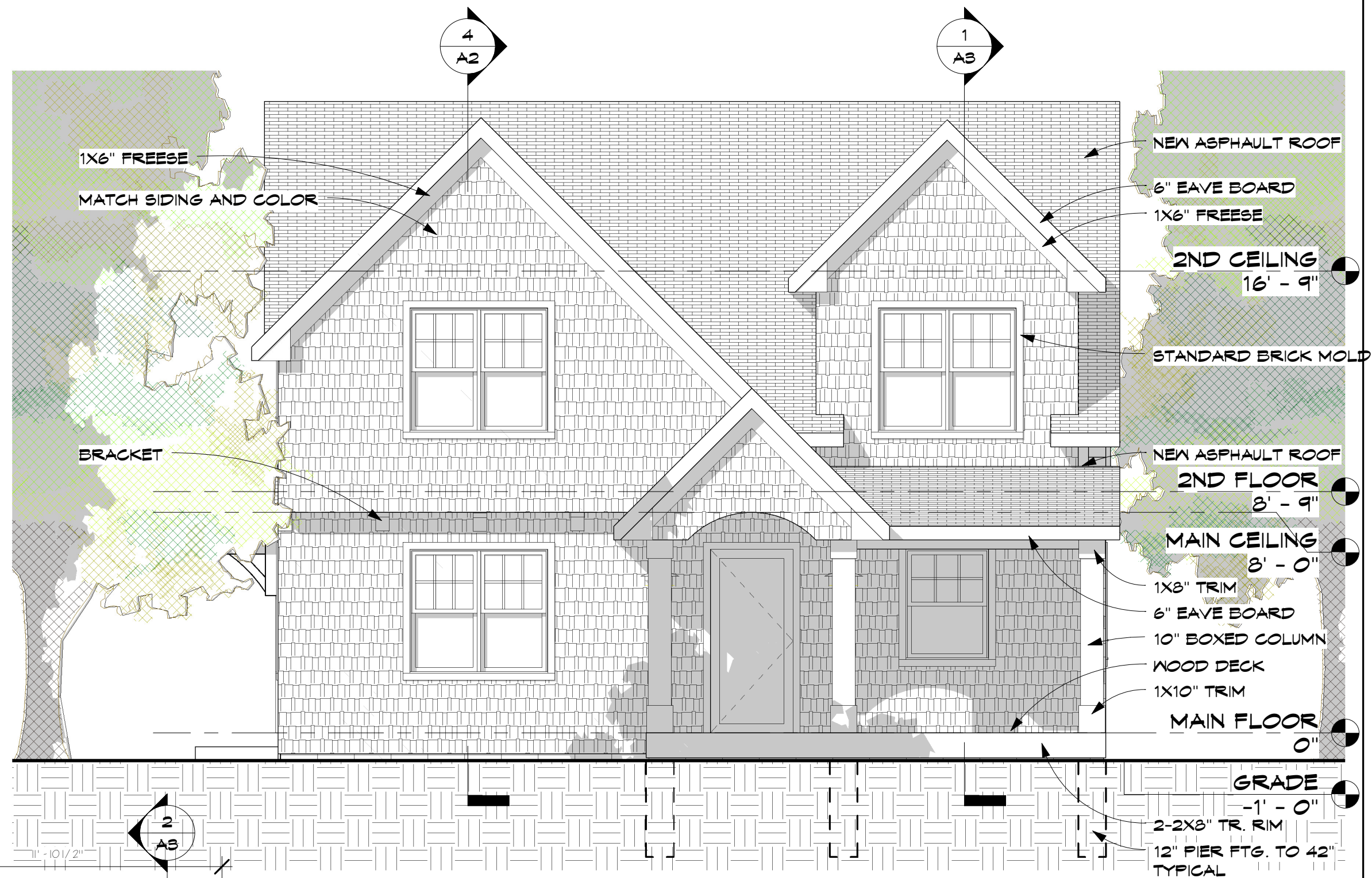
4 EAST A1 1/4" = 1'-0"
