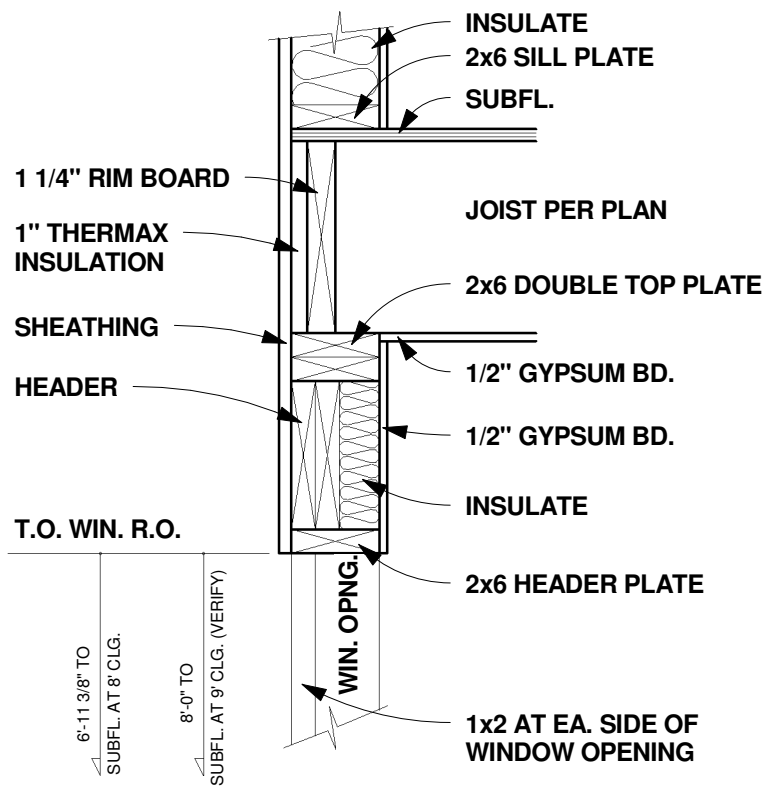
2 DETAIL AT TYPICAL HEADER A7 1" = 1'-0"
