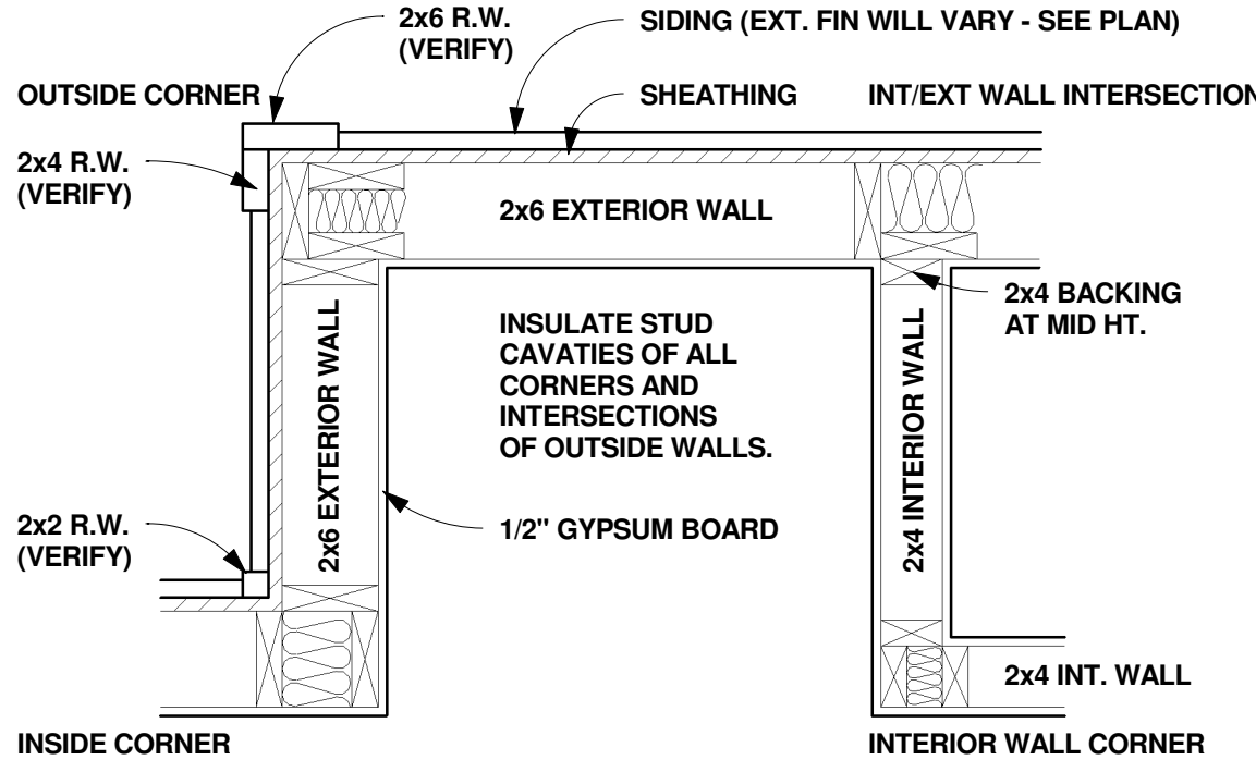
6 TYPICAL FRAMING DETAIL A7 1" = 1'-0"
