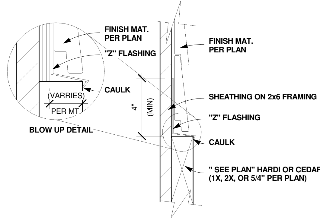
5 FLASHING DETAIL AT TRIM A7 3" = 1'-0"
