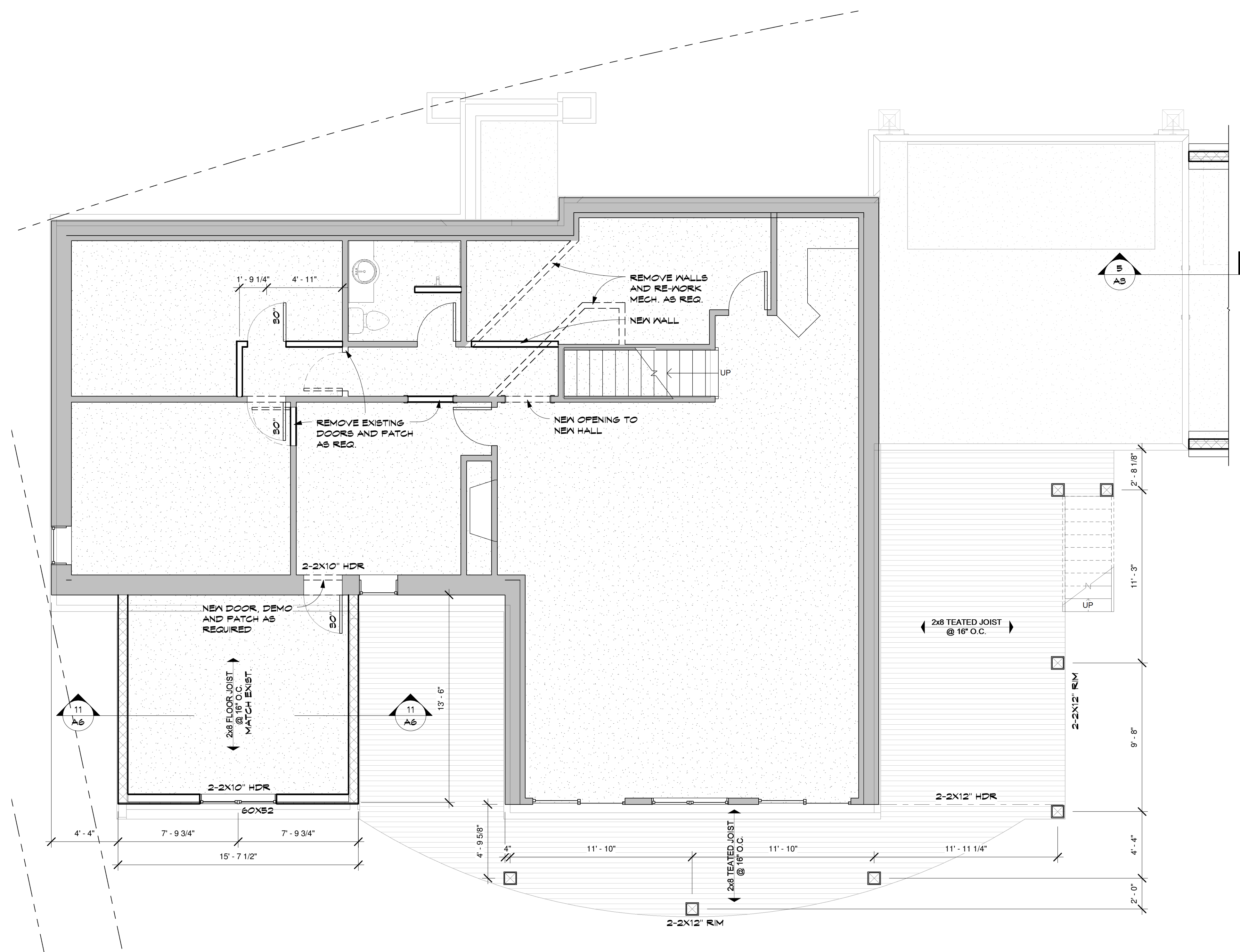
1 LOWER FLOOR A1 1/4" = 1'-0"
