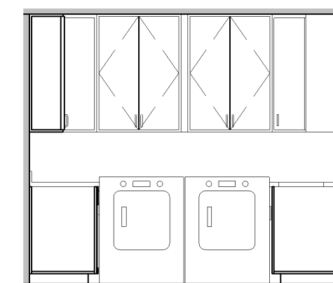
7 LAUNDRY 3 A6 1/4" = 1'-0"
