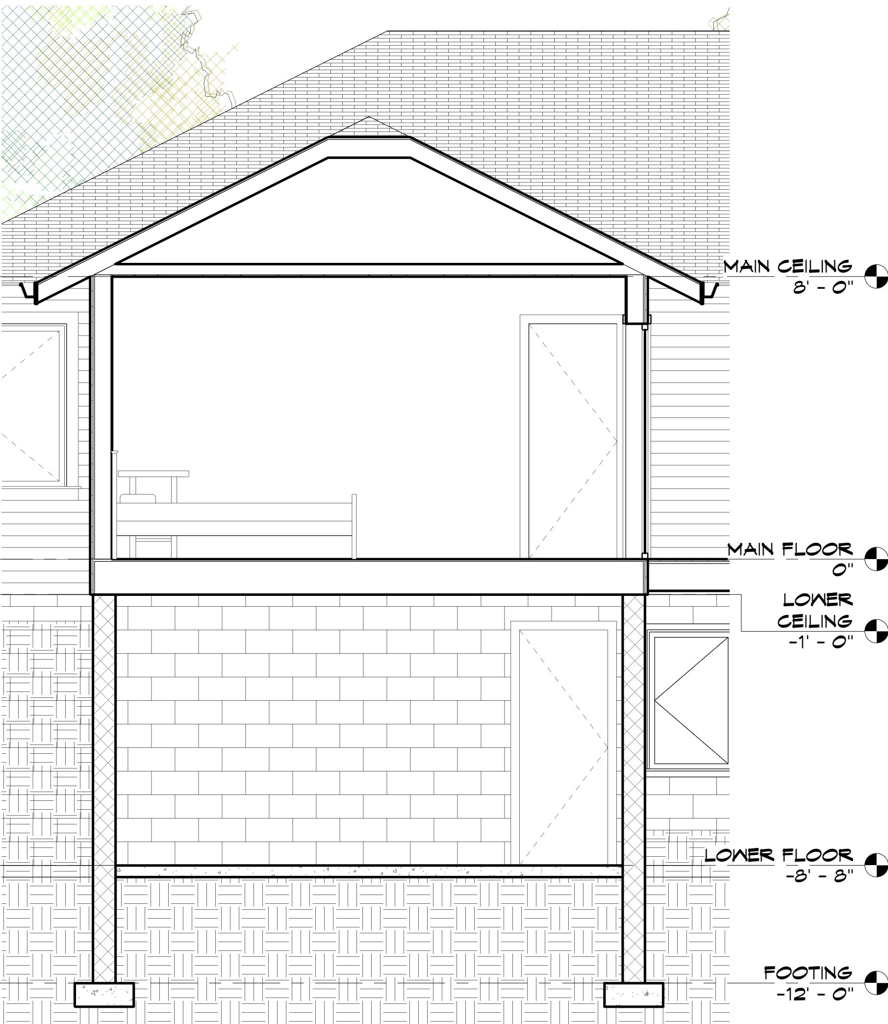
11 BUILDING SECTION A6 3/8" = 1'-0"
