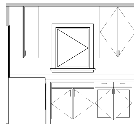
8 LAUNDRY 4 A6 1/4" = 1'-0"
